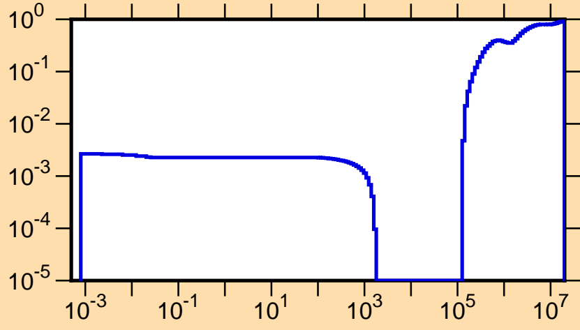
\mu vs. E for ^{250}\text{Cm}(\text{mt251})
