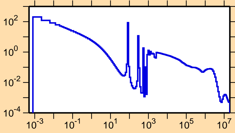
\sigma vs. E for ^{250}\text{Cm}(n,\gamma)
