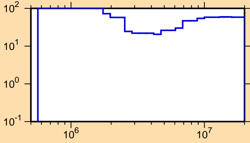
\Delta\sigma/\sigma vs. E for ^{250}\text{Cm}(n,ncont.)
