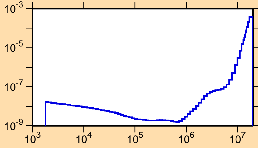
\sigma vs. E for ^{250}\text{Cm}(n,\alpha)
