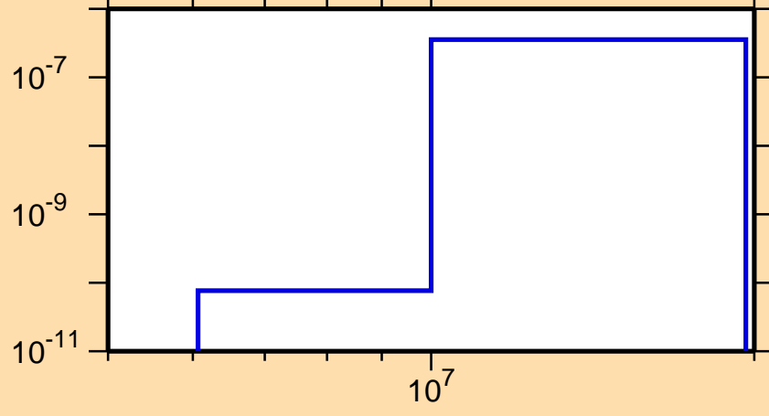
\sigma vs. E for ^{250}\text{Cm}(n,2n\alpha)
