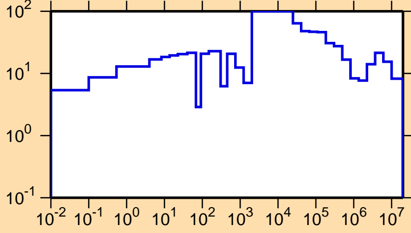
\Delta\sigma/\sigma vs. E for ^{250}\text{Cm}(n,tot.)
