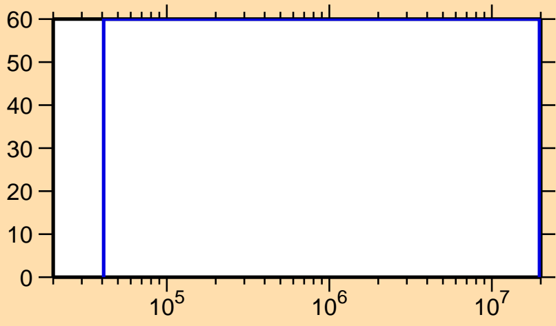
\Delta\sigma/\sigma vs. E for ^{250}\text{Cm}(n,f)
