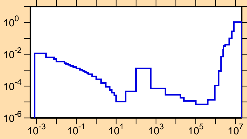
\sigma vs. E for ^{250}\text{Cm}(n,f)
