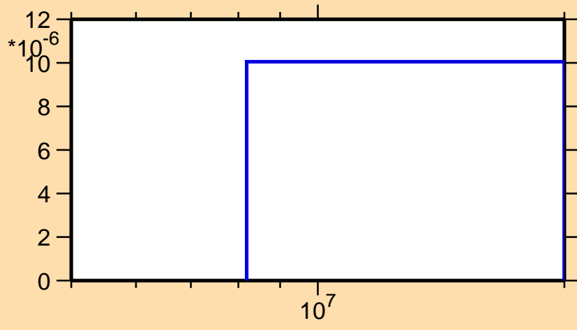
\sigma vs. E for ^{250}\text{Cm}(n,t)
