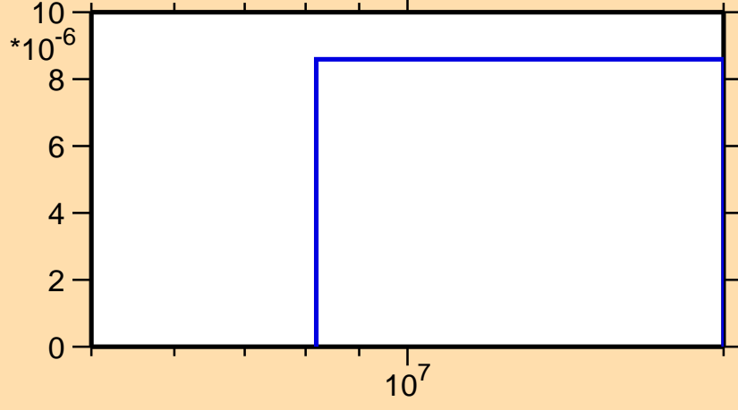
\sigma vs. E for ^{250}\text{Cm}(n,d)
