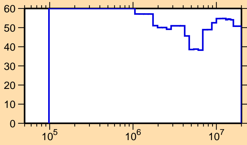
\Delta\sigma/\sigma vs. E for ^{251}\text{Cm}(n,ncont.)
