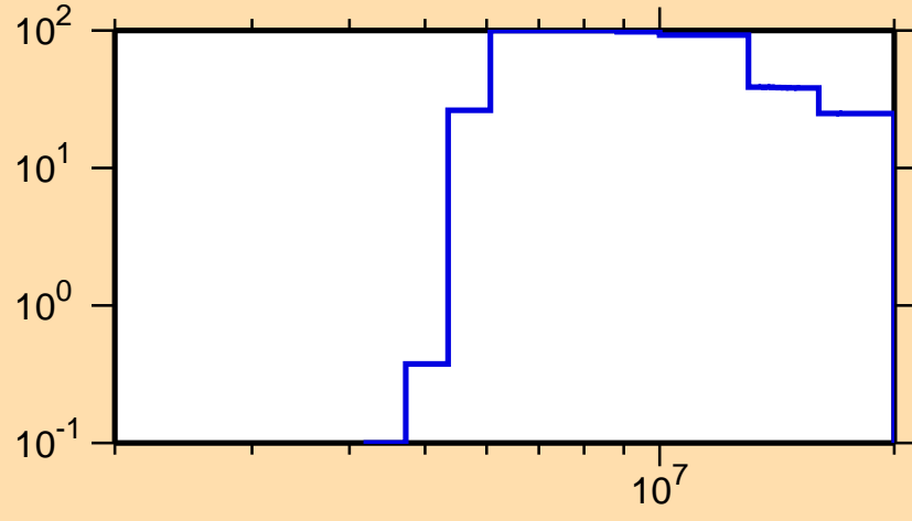
\Delta\sigma/\sigma vs. E for ^{251}\text{Cm}(n,p)
