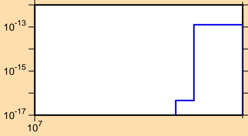
\sigma vs. E for ^{251}\text{Cm} (mt 11)
