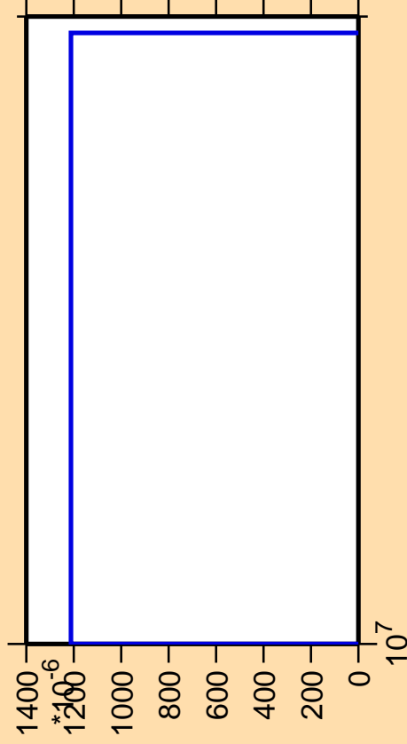
\Delta\sigma/\sigma vs. E for ^{251}\text{Cm} (mt 11)
