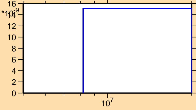
\sigma vs. E for ^{251}\text{Cm}(n,nd)
