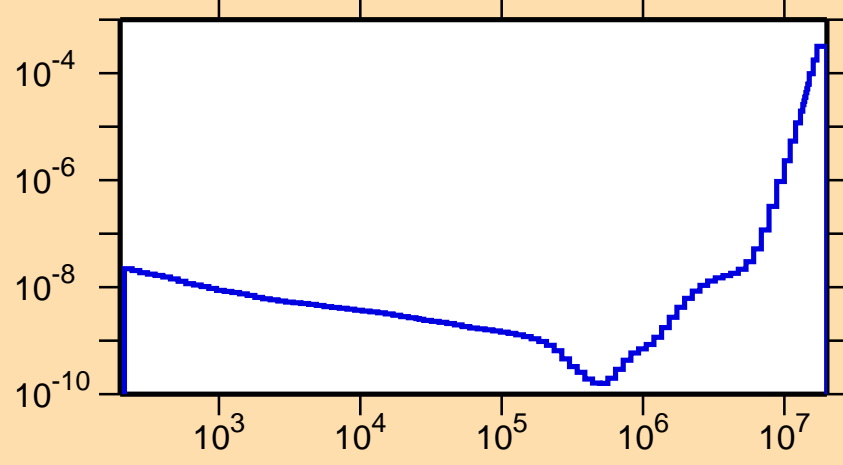
\sigma vs. E for ^{252}\text{Cm}(n,\alpha)
