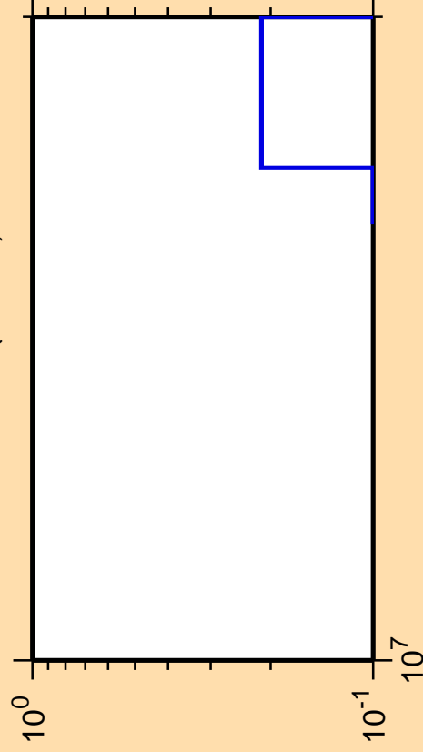
\Delta\sigma/\sigma vs. E for ^{252}\text{Cm} (mt 11)
