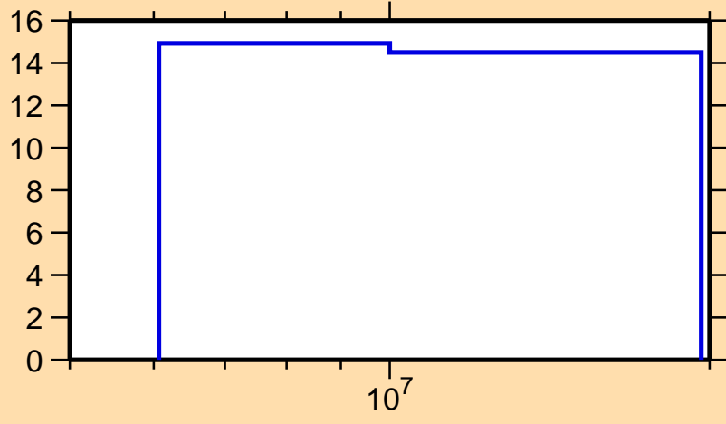
\Delta\sigma/\sigma vs. E for ^{252}\text{Cm}(n,\text{tot.})
