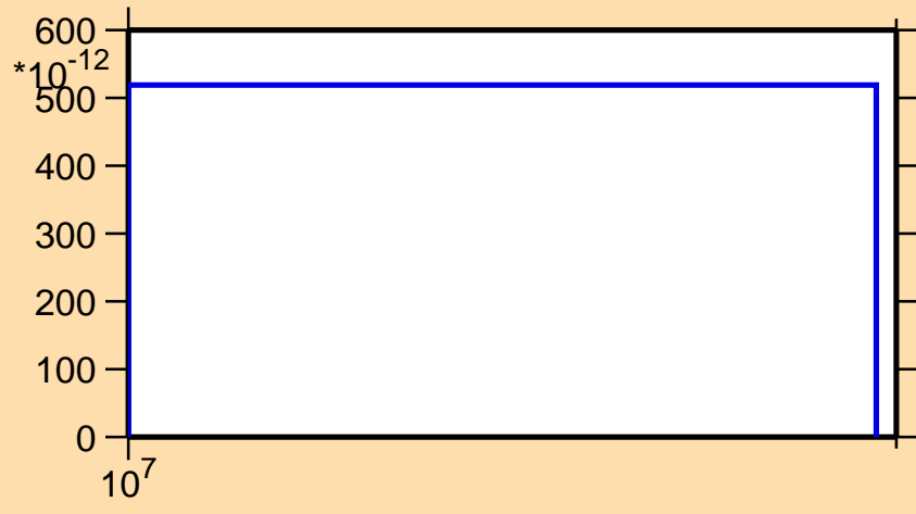
\sigma vs. E for ^{252}\text{Cm}(n,nd)
