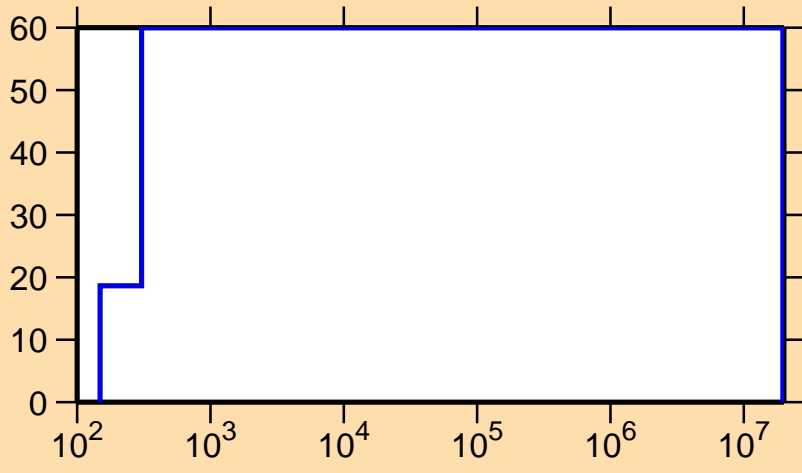
\Delta\sigma/\sigma vs. E for ^{252}\text{Cm}(n,\gamma)
