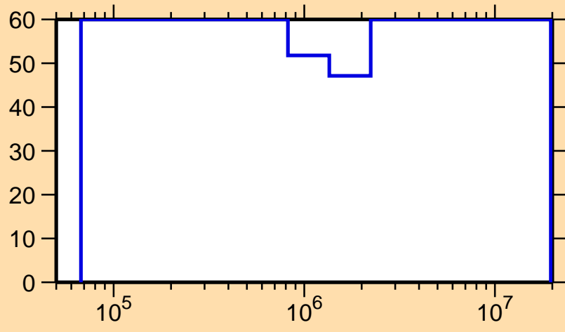
\Delta\sigma/\sigma vs. E for ^{252}\text{Cm}(n,n_1)
