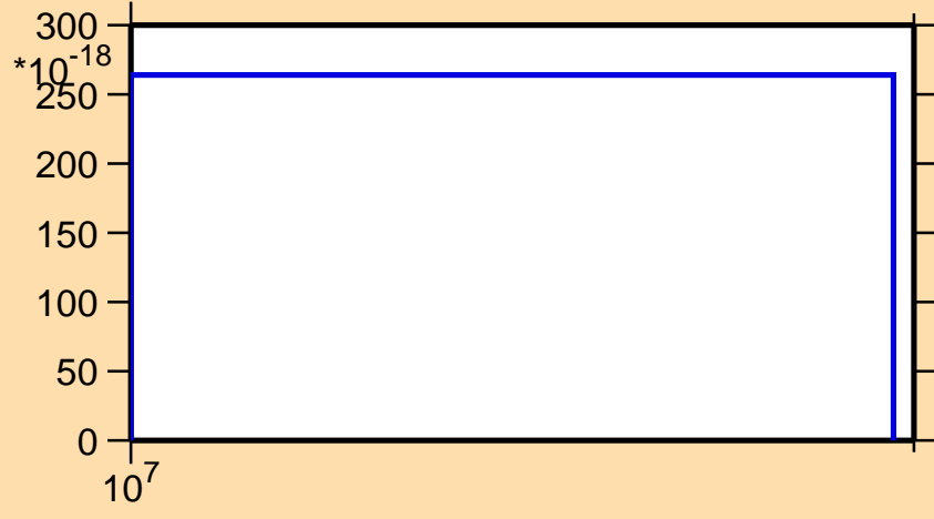
\sigma vs. E for ^{252}\text{Cm} (mt 11)
