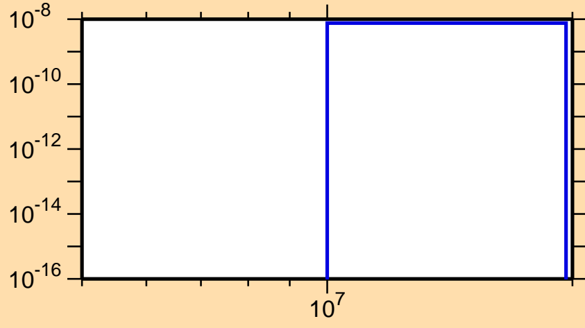
\sigma vs. E for ^{252}\text{Cm}(n,3n\alpha)
