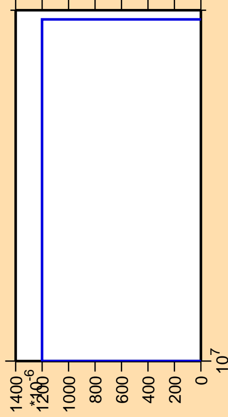
\Delta\sigma/\sigma vs. E for ^{252}\text{Cm} (mt 11)
