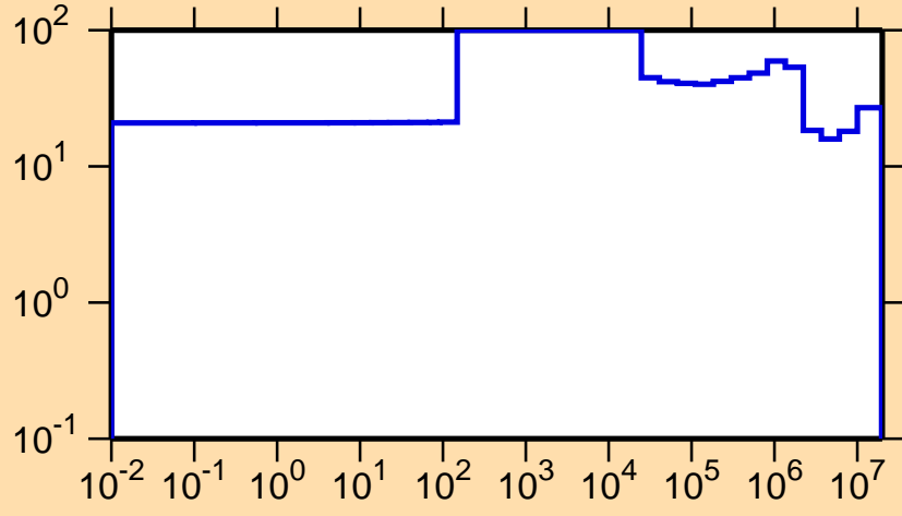
\Delta\sigma/\sigma vs. E for ^{252}\text{Cm}(n,el.)
