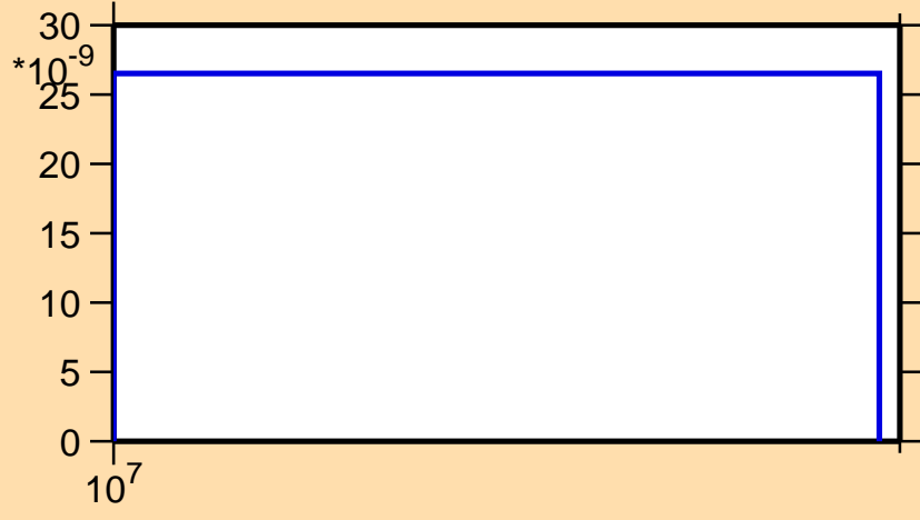
\sigma vs. E for ^{252}\text{Cm}(n,nt)
