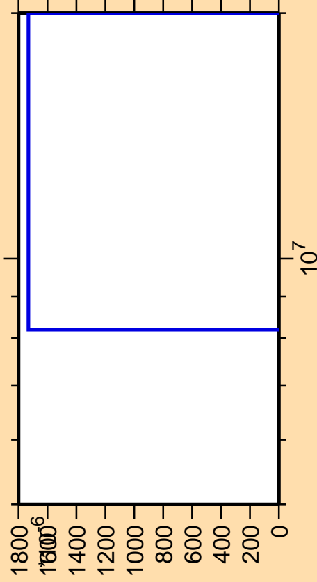
\Delta\sigma/\sigma vs. E for ^{252}\text{Cm}(\text{mt } 11)
