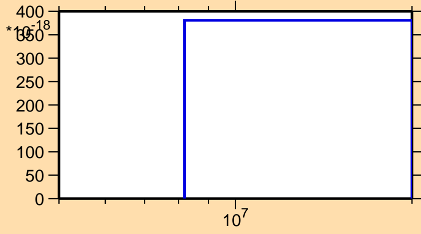
\sigma vs. E for ^{252}\text{Cm}(\text{mt } 11)
