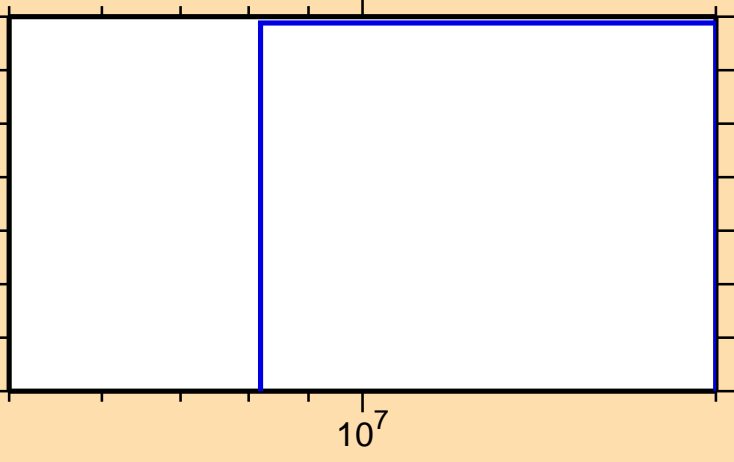
\sigma vs. E for ^{252}\text{Cm}(n,d)
