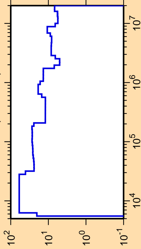
\Delta\sigma/\sigma vs. E for ^{54}\text{Co}(n,\text{nonel.})
