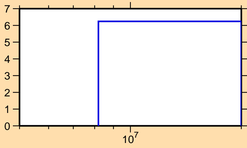
\Delta\sigma/\sigma vs. E for ^{54}\text{Co}(n,\text{nonel.})
