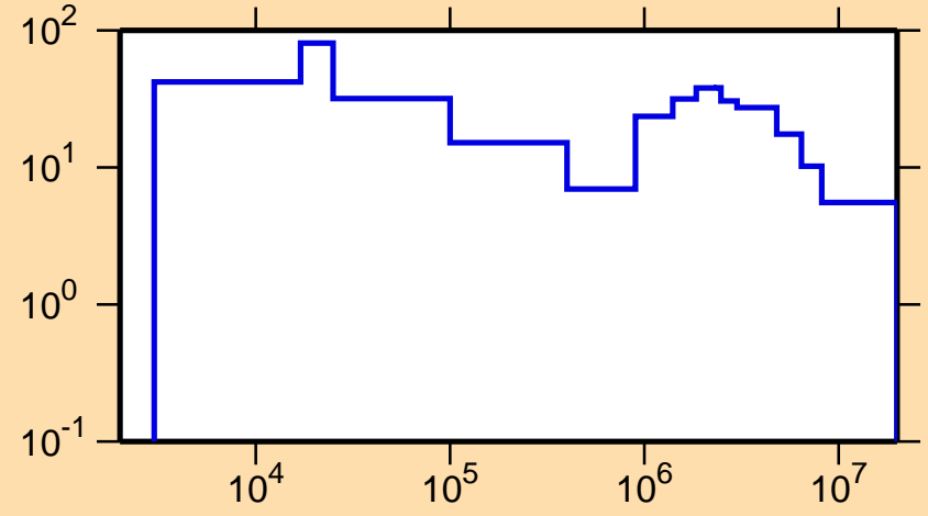
\Delta\sigma/\sigma vs. E for ^{54}\text{Co}(n,\text{el.})
