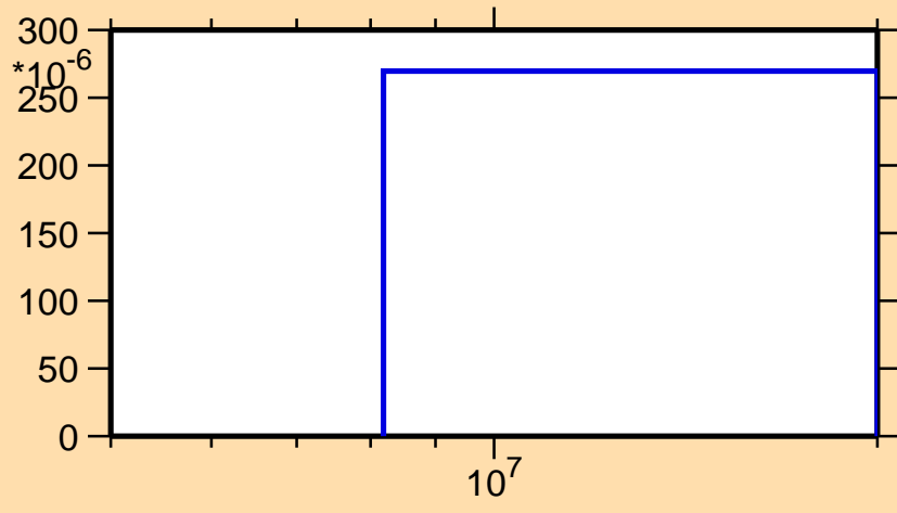
\sigma vs. E for ^{54}\text{Co}(n,\text{pd})
