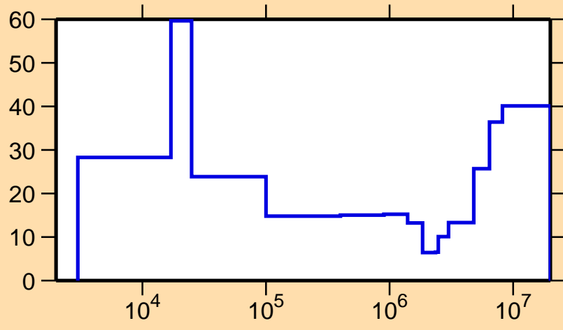
\Delta\sigma/\sigma vs. E for ^{54}\text{Co}(n,p)
