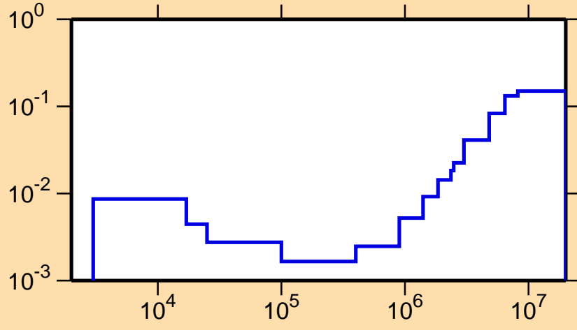
\sigma vs. E for ^{54}\text{Co}(n,\alpha)
