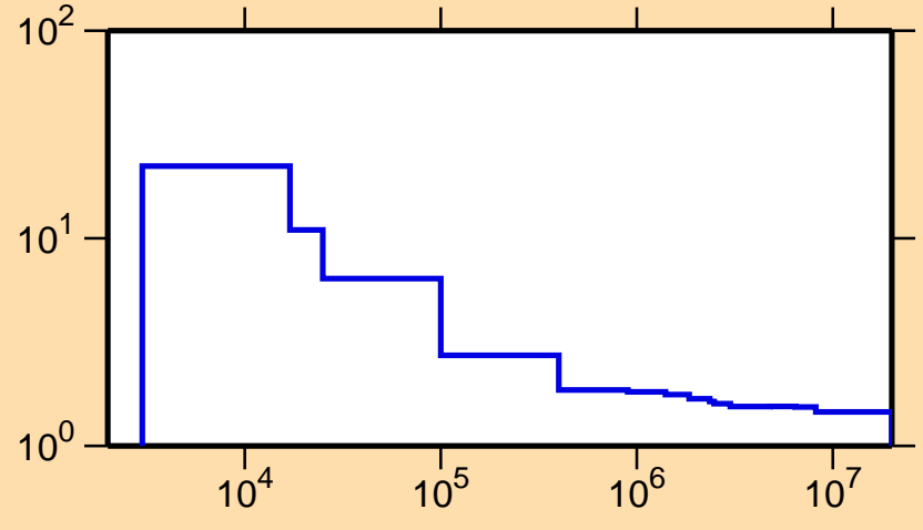
\sigma vs. E for ^{54}\text{Co}(n,\text{nonel.})
