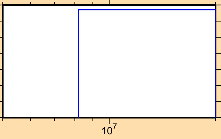
\sigma vs. E for ^{54}\text{Co}(n,\text{nd})
