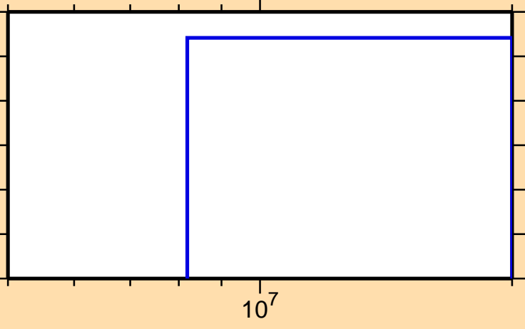
\sigma vs. E for ^{54}\text{Co}(n,2n)
