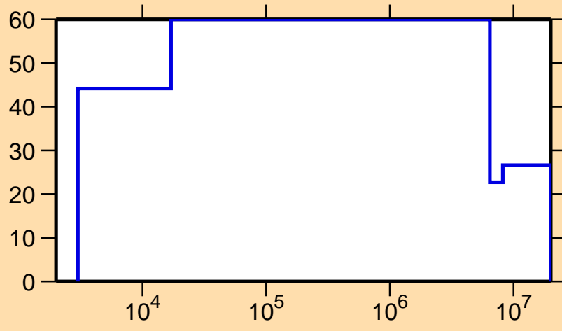
\Delta\sigma/\sigma vs. E for ^{54}\text{Co}(n,\gamma)
