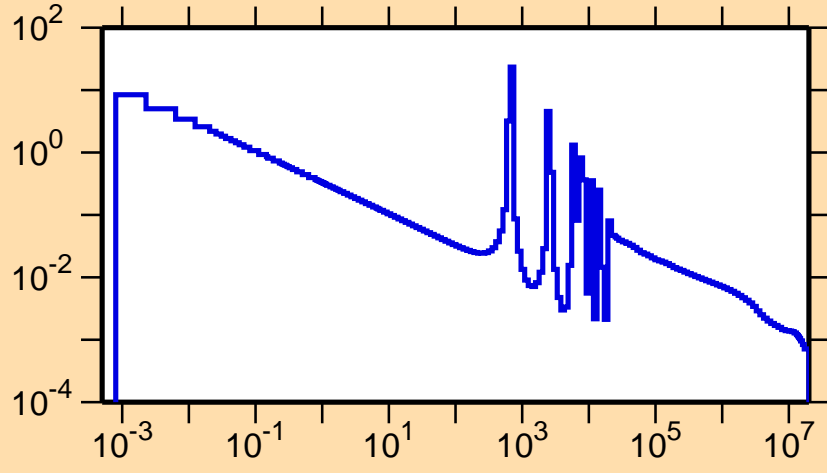
\sigma vs. E for ^{55}\text{Co}(n,\gamma)
