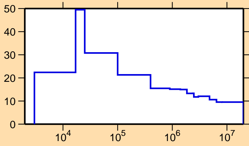
\Delta\sigma/\sigma vs. E for ^{55}\text{Co}(n,\text{nonel.})
