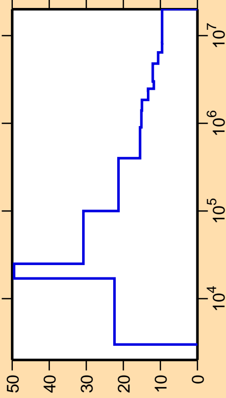
\Delta\sigma/\sigma vs. E for ^{55}\text{Co}(n,\text{nonel.})
