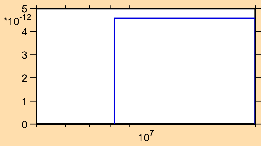
\sigma vs. E for ^{55}\text{Co} (mt 45)
