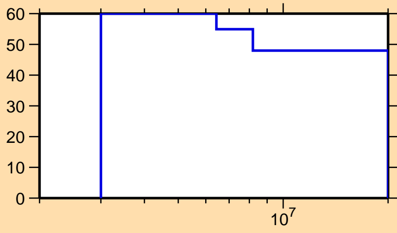
\Delta\sigma/\sigma vs. E for ^{55}\text{Co}(n,n\text{cont.})
