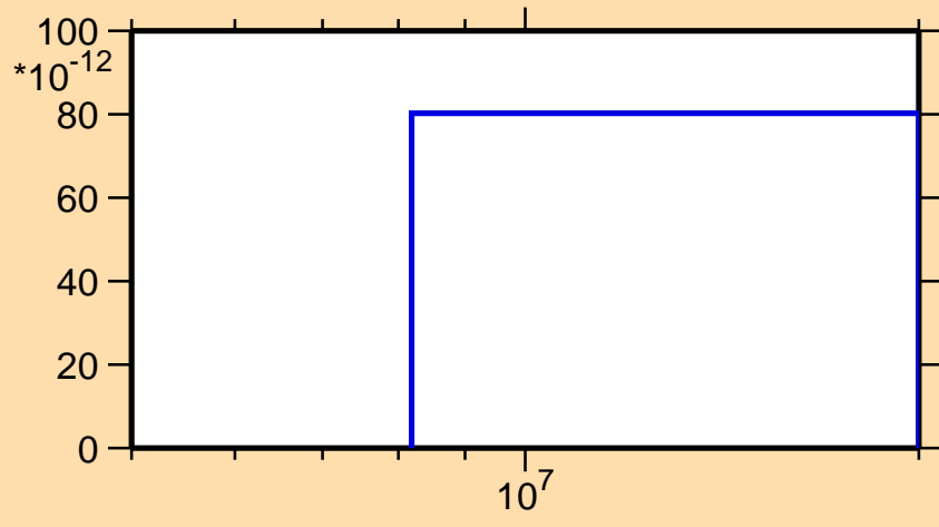
\sigma vs. E for ^{55}\text{Co}(n,2np)
