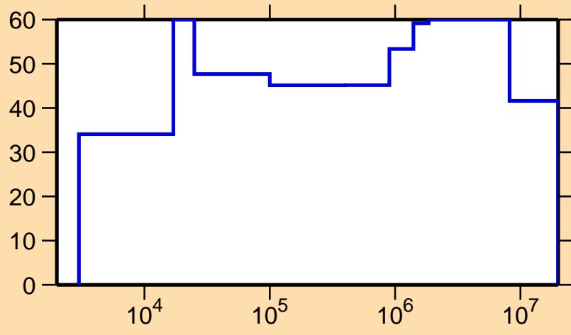
\Delta\sigma/\sigma vs. E for ^{55}\text{Co}(n,\gamma)
