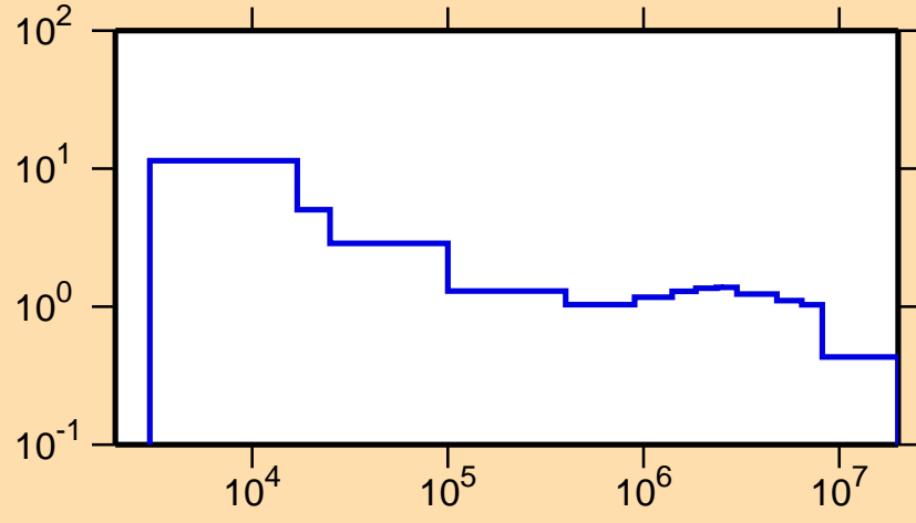
\sigma vs. E for ^{55}\text{Co}(n,p)
