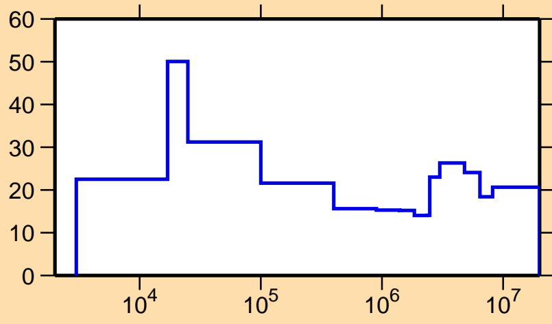
\Delta\sigma/\sigma vs. E for ^{55}\text{Co}(n,p)
