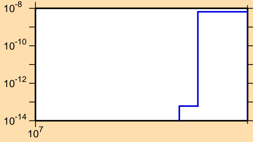
\sigma vs. E for ^{56}\text{Co}(n,\text{pt})
