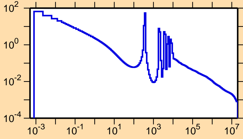
\sigma vs. E for ^{56}\text{Co}(n,\gamma)
