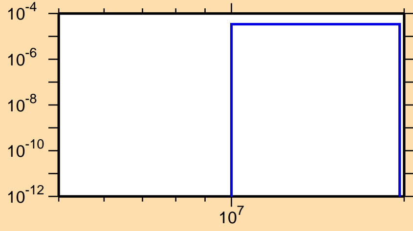
\sigma vs. E for ^{56}\text{Co}(n,\text{He}3)
