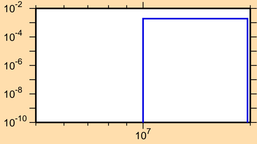
\sigma vs. E for ^{56}\text{Co}(n,n\alpha)
