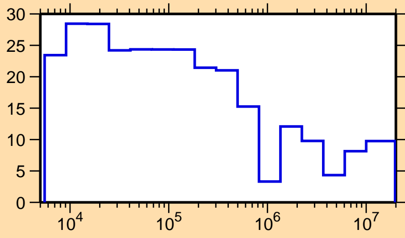
\Delta\sigma/\sigma vs. E for ^{56}\text{Co}(n,el.)
