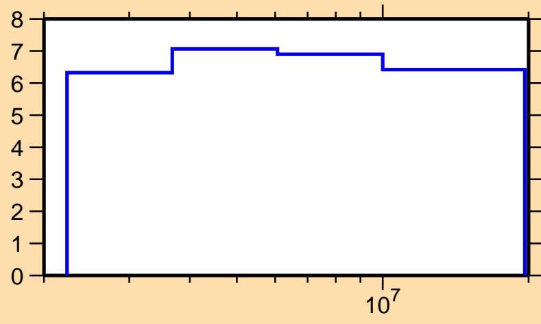
\Delta\sigma/\sigma vs. E for ^{56}\text{Co}(n,n\text{nonel.})
