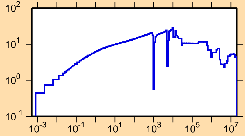
\Delta\sigma/\sigma vs. E for ^{57}\text{Co}(n,\text{tot.})
