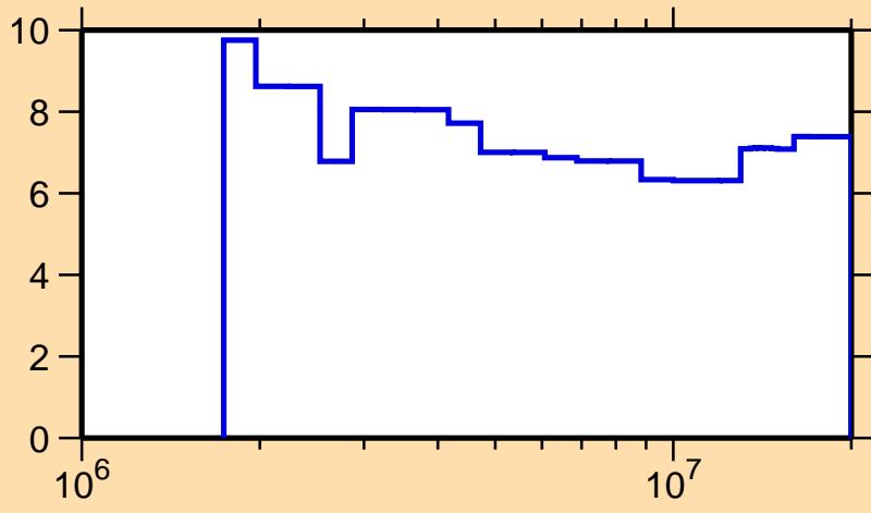
\Delta\sigma/\sigma vs. E for ^{58}\text{Co}(n,n\text{nonel.})
