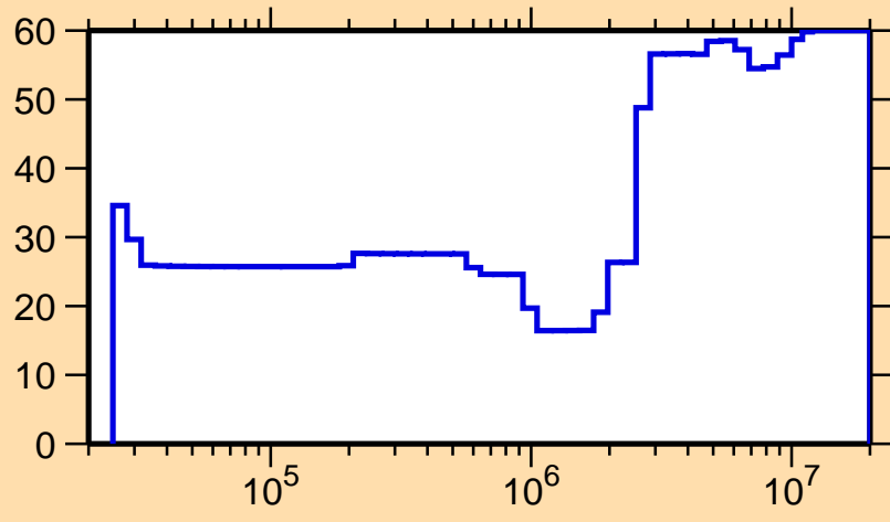
\Delta\sigma/\sigma vs. E for ^{58}\text{Co}(n,n_1)
