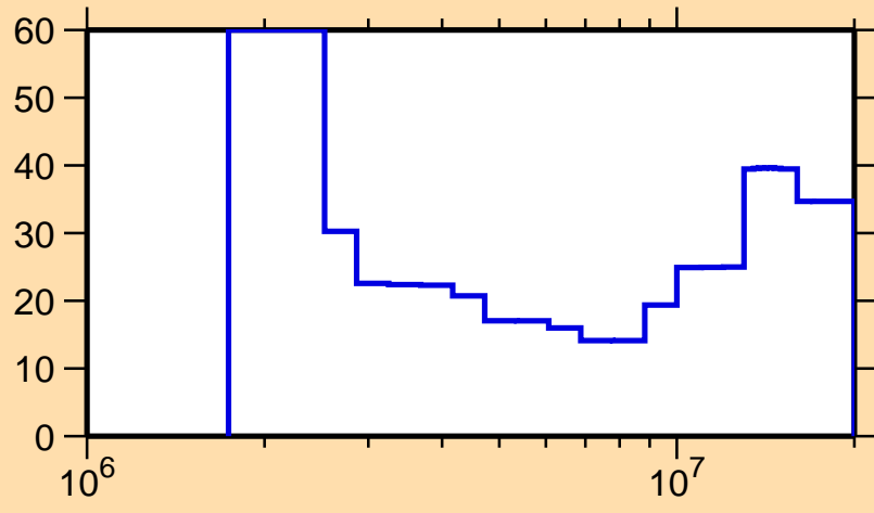
\Delta\sigma/\sigma vs. E for ^{58}\text{Co}(n,ncont.)
