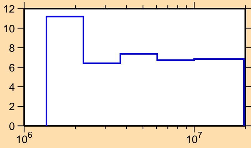
\Delta\sigma/\sigma vs. E for ^{58}\text{Co}(n,n\text{onel.})
