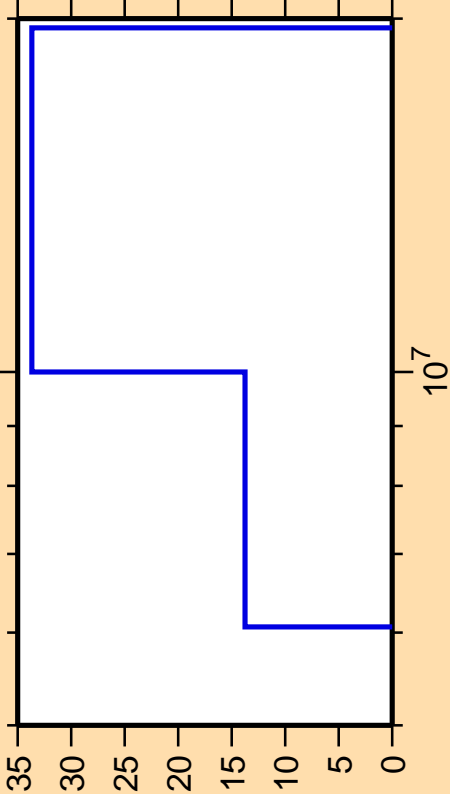
\Delta\sigma/\sigma vs. E for ^{58}\text{Co}(n,n\text{cont.})
