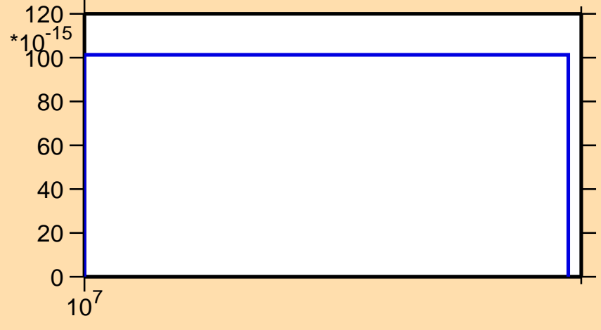
\sigma vs. E for ^{58}\text{Co} (mt117)
