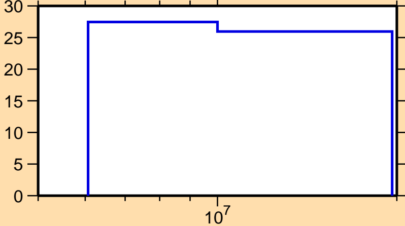
\Delta\sigma/\sigma vs. E for ^{58}\text{Co}(n,2n)
