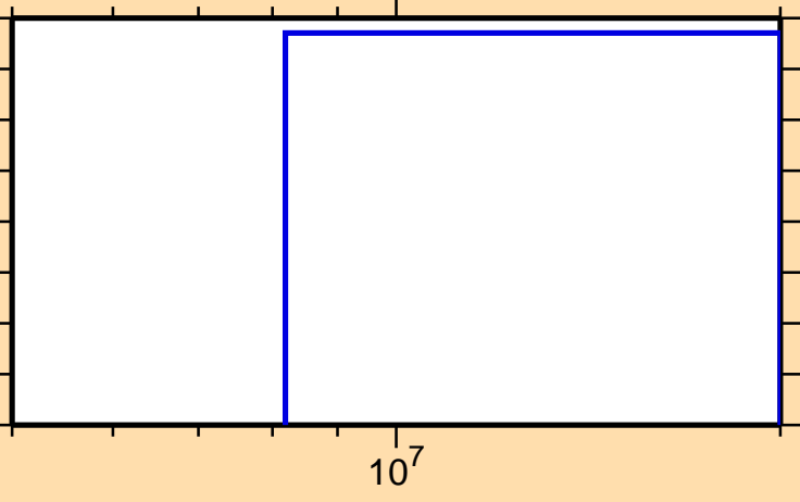
\sigma vs. E for ^{58}\text{Co}(n,\text{nd})
