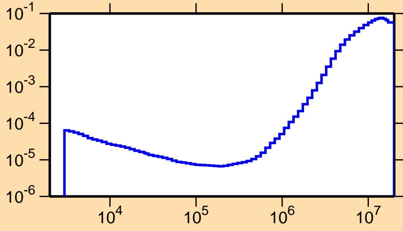
\sigma vs. E for ^{58}\text{Co}(n,\alpha)
