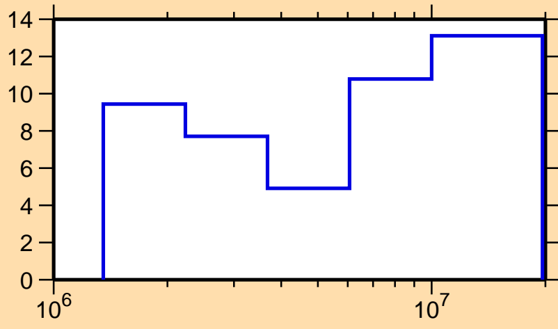
\Delta\sigma/\sigma vs. E for ^{58}\text{Co}(n, el.)
