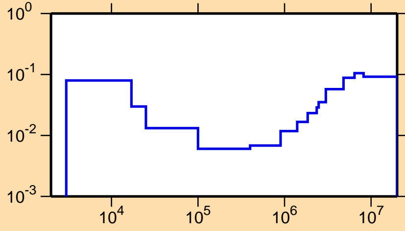
\sigma vs. E for ^{58}\text{Co}(n,p)
