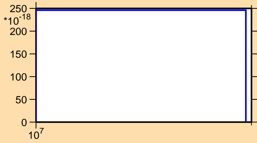
\sigma vs. E for ^{59}\text{Co} (mt 45)
