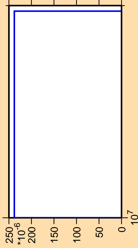
\Delta\sigma/\sigma vs. E for ^{59}\text{Co} (mt 45)
