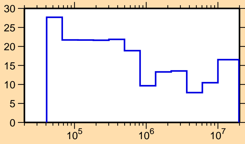
\Delta\sigma/\sigma vs. E for ^{60}\text{Co}(n,el.)
