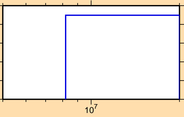
\sigma vs. E for ^{60}\text{Co}(n,2np)
