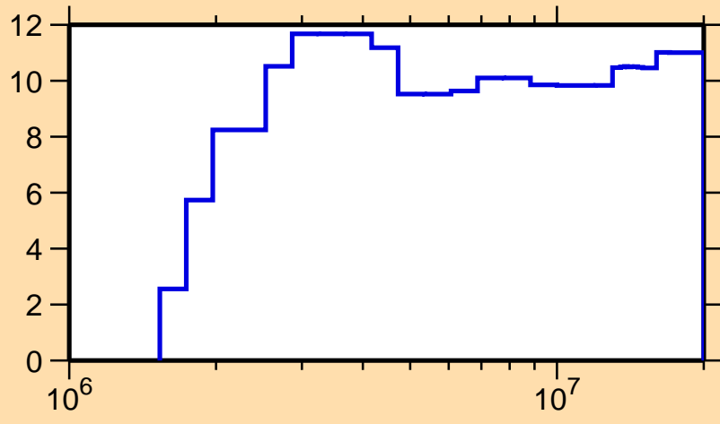
\Delta\sigma/\sigma vs. E for ^{60}\text{Co}(n,n\text{nonel.})
