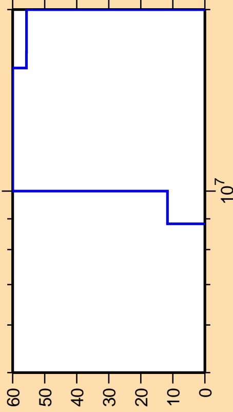
\Delta\sigma/\sigma vs. E for ^{60}\text{Co}(n,n\alpha)
