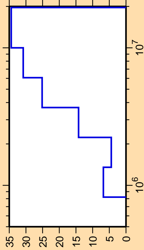
\Delta\sigma/\sigma vs. E for ^{61}\text{Co}(n,n_4)
