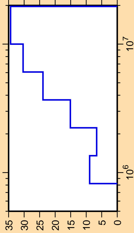
\Delta\sigma/\sigma vs. E for ^{61}\text{Co}(n,n_1)
