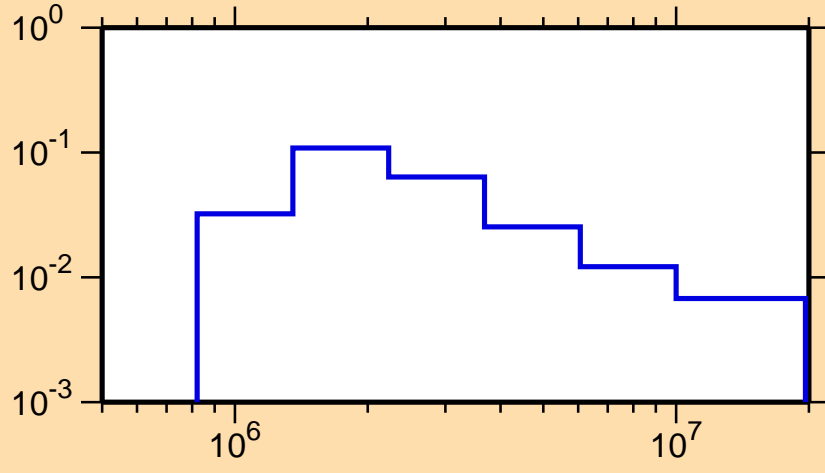
\sigma vs. E for ^{61}\text{Co}(n,n_1)
