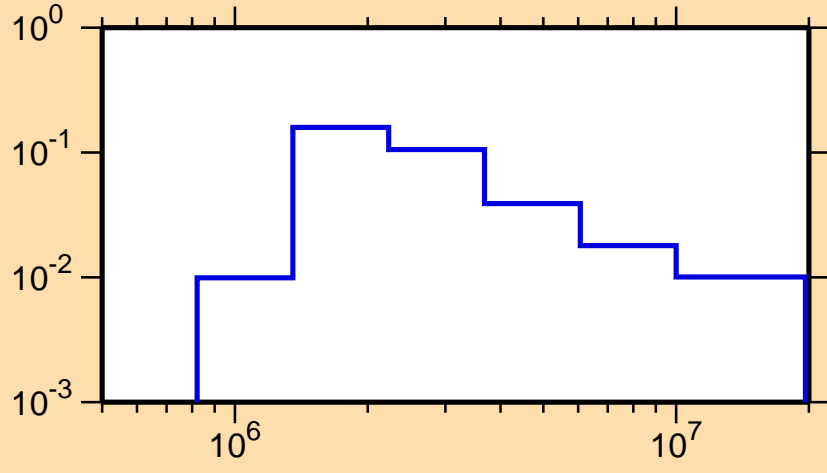
\sigma vs. E for ^{61}\text{Co}(n,n_2)
