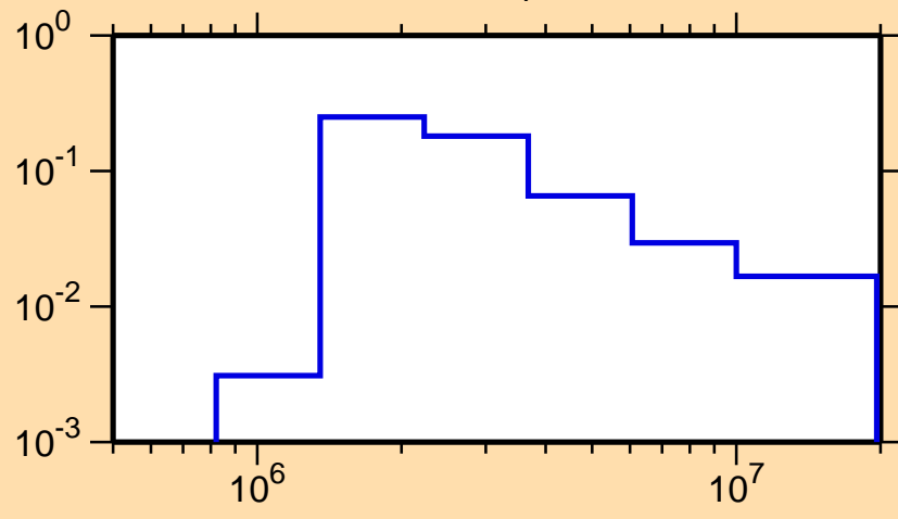
\sigma vs. E for ^{61}\text{Co}(n,n_4)
