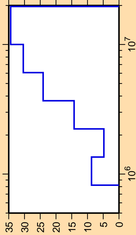
\Delta\sigma/\sigma vs. E for ^{61}\text{Co}(n,n_2)
