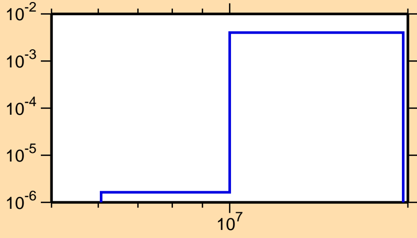
\sigma vs. E for ^{61}\text{Co}(n,d)
