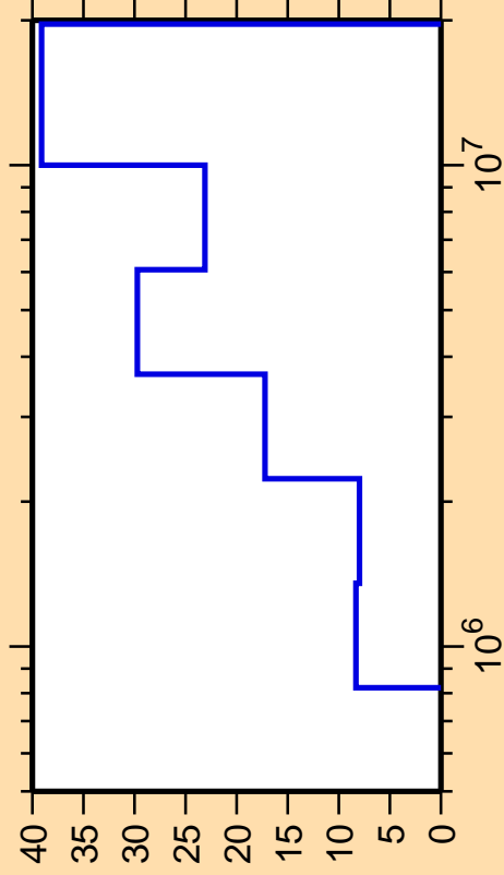
\Delta\sigma/\sigma vs. E for ^{61}\text{Co}(n,n_3)
