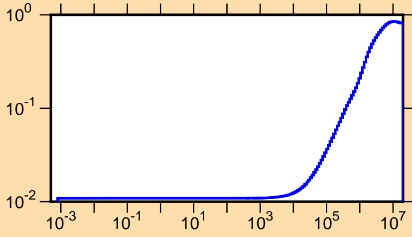
\mu vs. E for ^{62}\text{Co}(\text{mt251})
