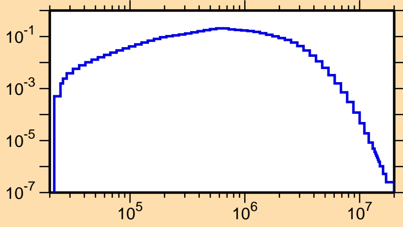
\sigma vs. E for ^{62}\text{Co}(n,n_1)
