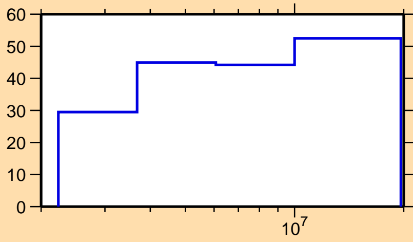
\Delta\sigma/\sigma vs. E for ^{62}\text{Co}(n,n_1)
