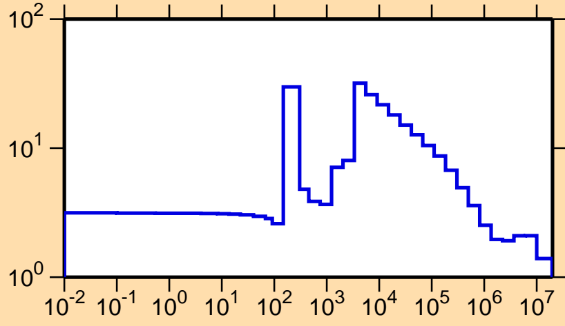
\sigma vs. E for ^{62}\text{Co}(n,\text{el.})
