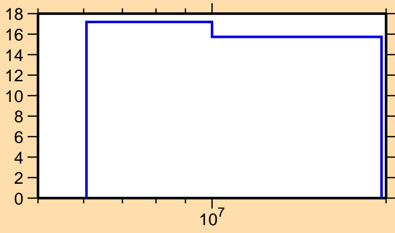
\Delta\sigma/\sigma vs. E for ^{62}\text{Co}(n,2n)
