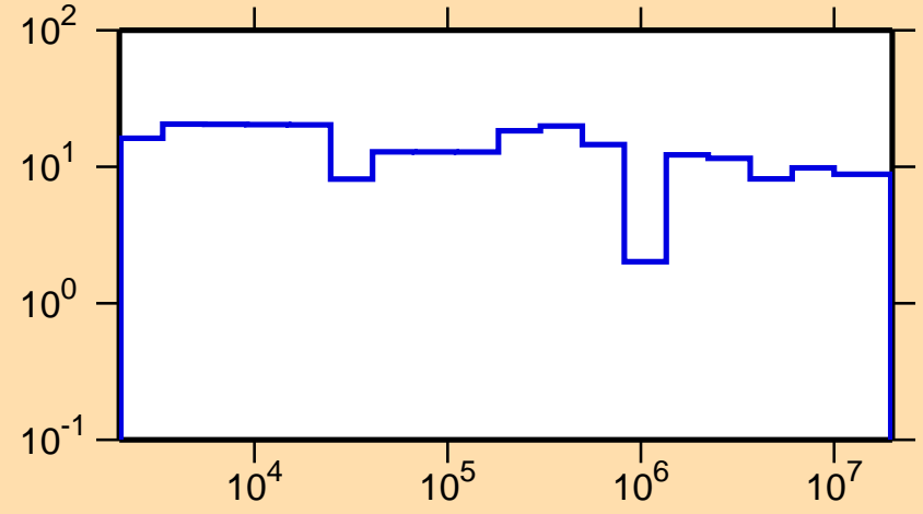
\Delta\sigma/\sigma vs. E for ^{62}\text{Co}(n,\text{el.})
