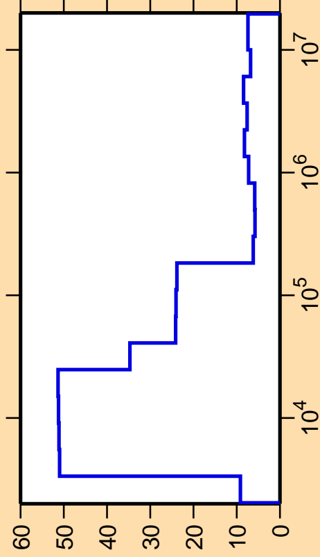
\Delta\sigma/\sigma vs. E for ^{62}\text{Co}(n,\text{nonel.})
