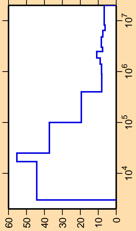
\Delta\sigma/\sigma vs. E for ^{62}\text{Co}(n,\text{nonel.})
