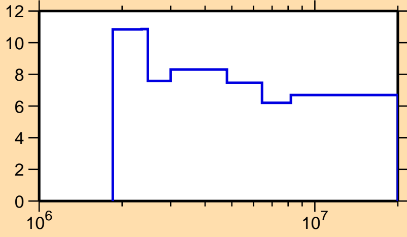
\Delta\sigma/\sigma vs. E for ^{62}\text{Co}(n,n\text{onel.})
