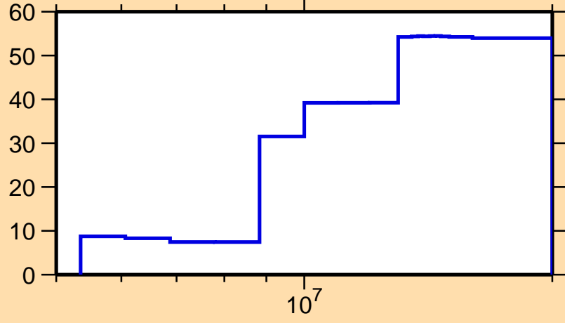
\Delta\sigma/\sigma vs. E for ^{63}\text{Co}(n,n\text{cont.})
