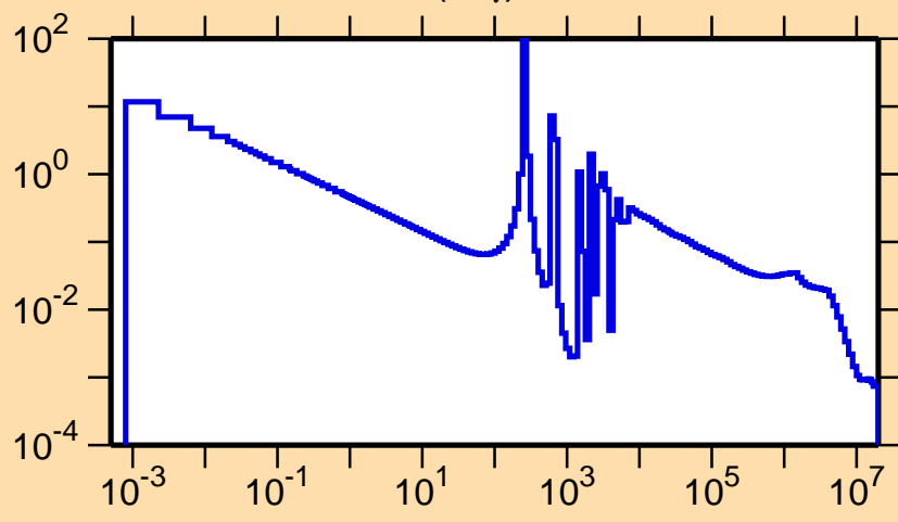
\sigma vs. E for ^{63}\text{Co}(n,\gamma)
