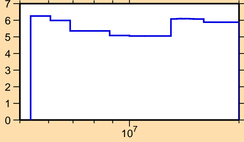
\Delta\sigma/\sigma vs. E for ^{63}\text{Co}(n,\text{nonel.})
