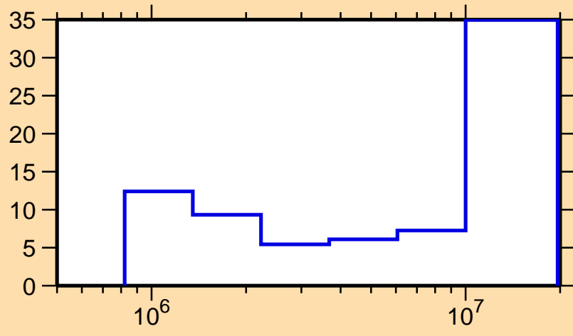
\Delta\sigma/\sigma vs. E for ^{63}\text{Co}(n,\text{inel.})
