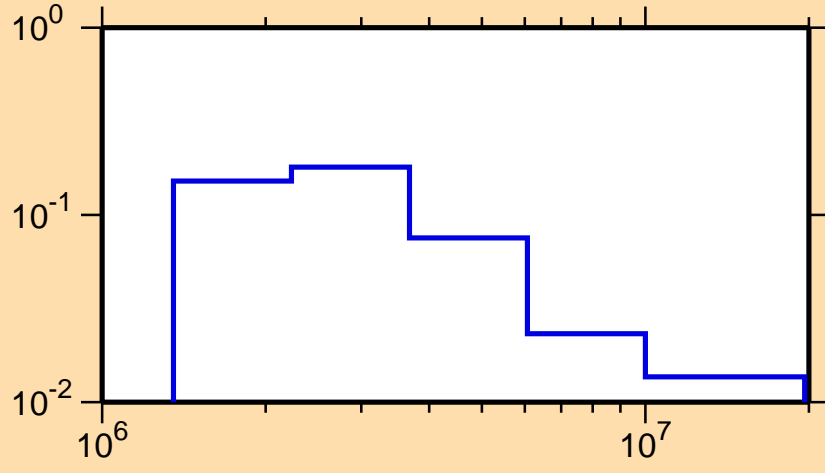
\sigma vs. E for ^{63}\text{Co}(n,n_3)
