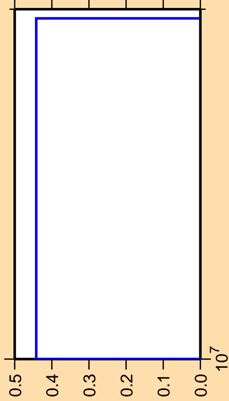
\Delta\sigma/\sigma vs. E for ^{63}\text{Co}(n,2np)
