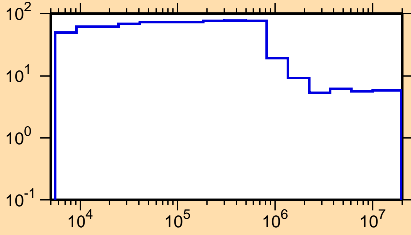
\Delta\sigma/\sigma vs. E for ^{63}\text{Co}(n,\text{nonel.})
