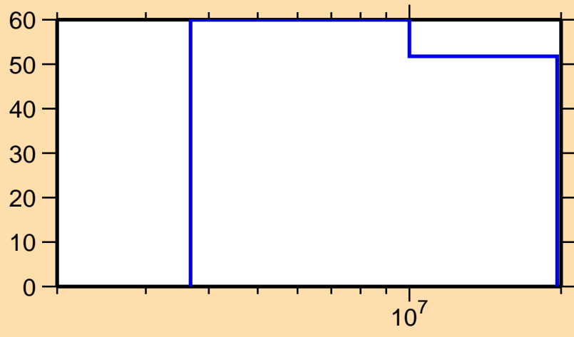
\Delta\sigma/\sigma vs. E for ^{63}\text{Co}(n,\gamma)
