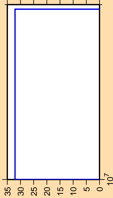
\Delta\sigma/\sigma vs. E for ^{63}\text{Co}(n,3n)
