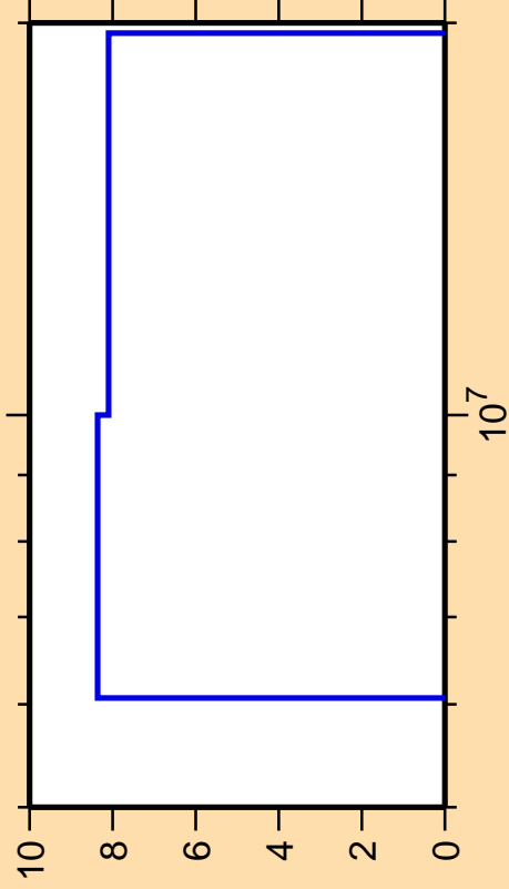
\Delta\sigma/\sigma vs. E for ^{63}\text{Co}(n,2n)
