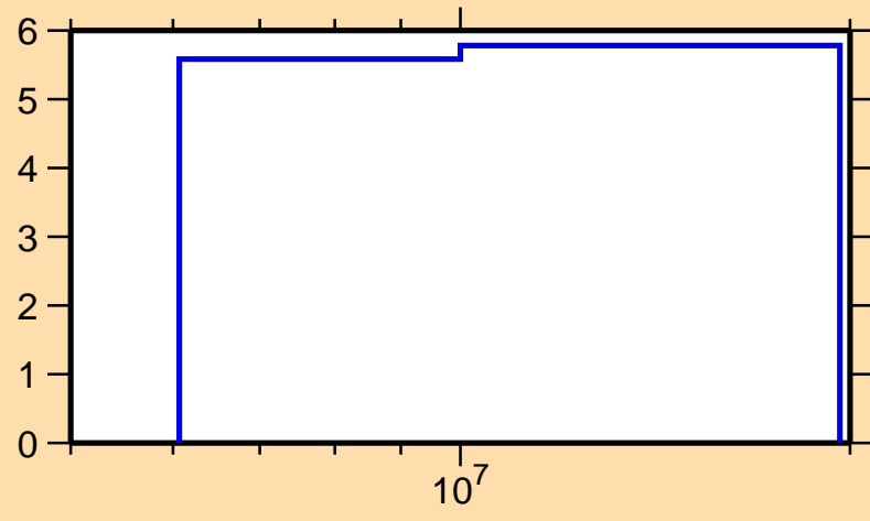
\Delta\sigma/\sigma vs. E for ^{63}\text{Co}(n,\text{nonel.})
