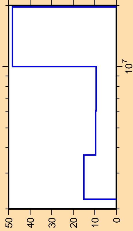
\Delta\sigma/\sigma vs. E for ^{63}\text{Co}(n,n\text{cont.})
