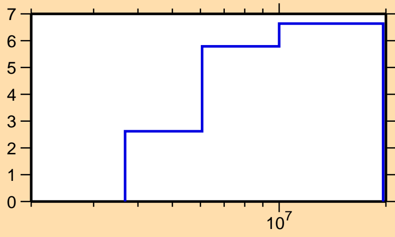
\Delta\sigma/\sigma vs. E for ^{63}\text{Co}(n,\text{tot.})
