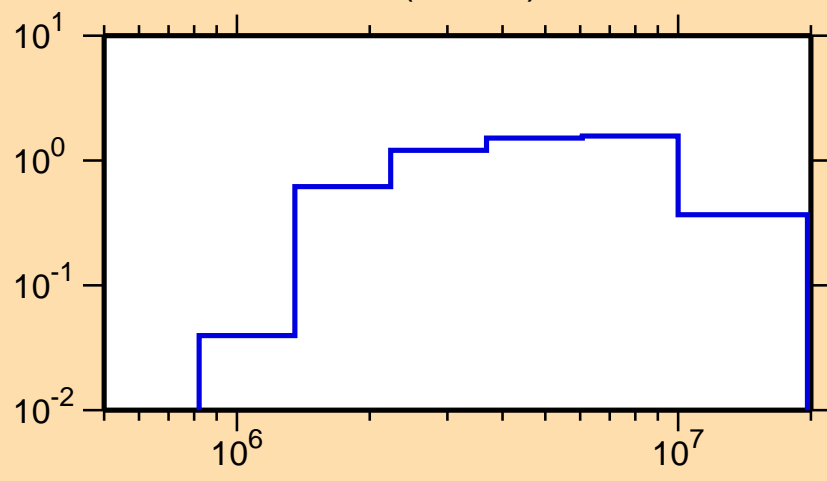
\sigma vs. E for ^{63}\text{Co}(n,\text{inel.})
