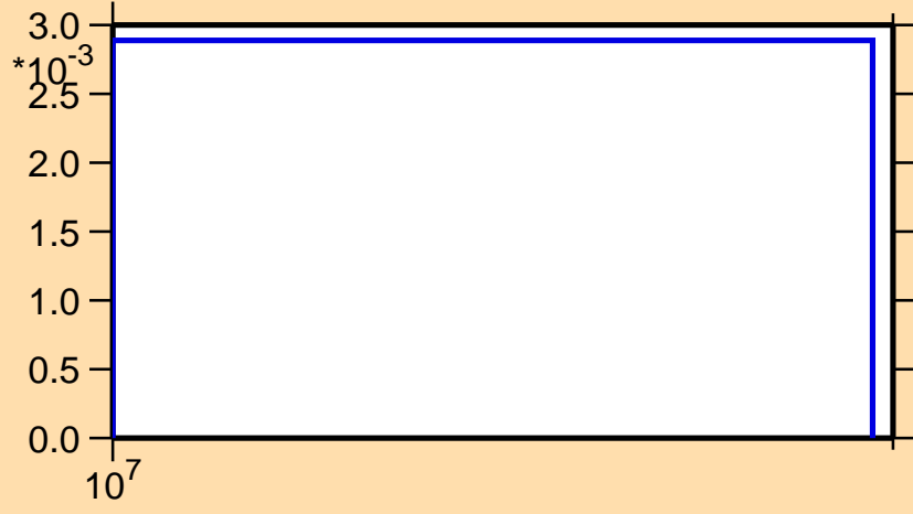
\sigma vs. E for ^{63}\text{Co}(n,3n)
