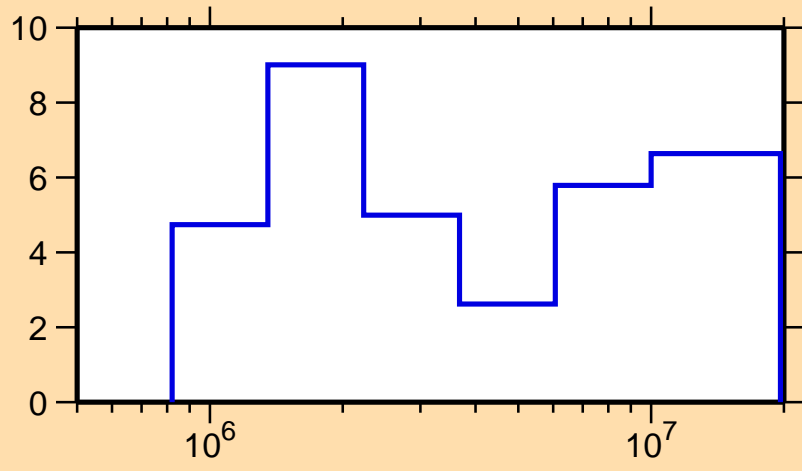
\Delta\sigma/\sigma vs. E for ^{63}\text{Co}(n,\text{tot.})
