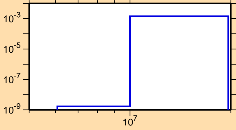
\sigma vs. E for ^{63}\text{Co}(n,d)
