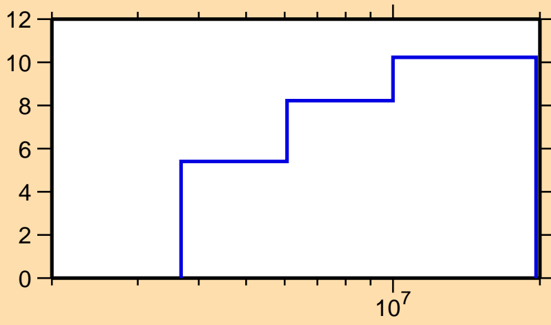
\Delta\sigma/\sigma vs. E for ^{63}\text{Co}(n,\text{el.})
