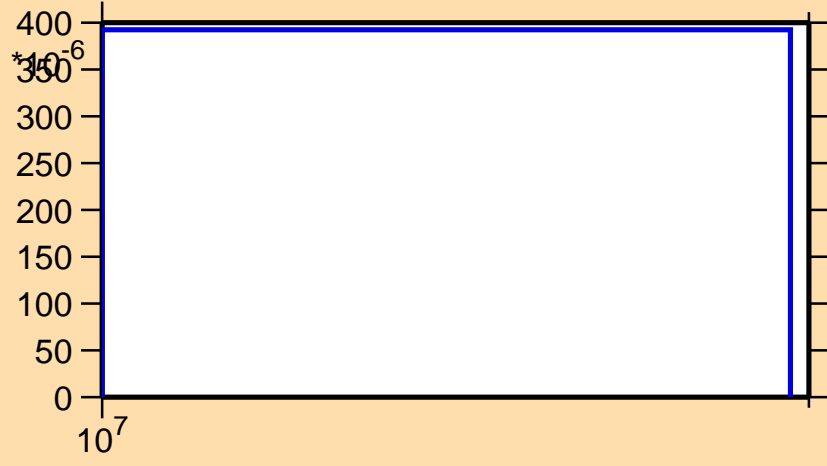
\sigma vs. E for ^{63}\text{Co}(n,np)
