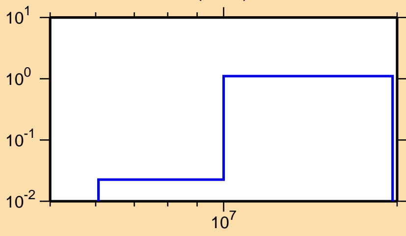
\sigma vs. E for ^{63}\text{Co}(n,2n)
