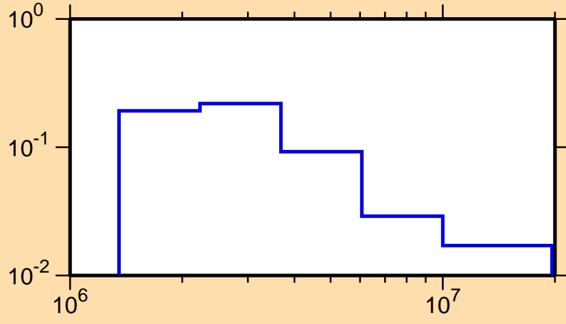
\sigma vs. E for ^{63}\text{Co}(n,n_2)
