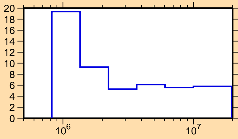
\Delta\sigma/\sigma vs. E for ^{63}\text{Co}(n,\text{nonel.})
