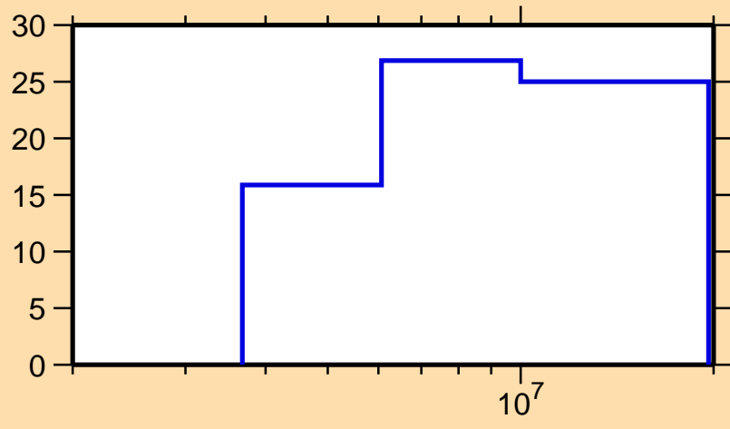
\Delta\sigma/\sigma vs. E for ^{63}\text{Co}(n,n_1)
