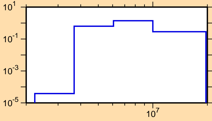
\sigma vs. E for ^{63}\text{Co}(n,n\text{cont.})
