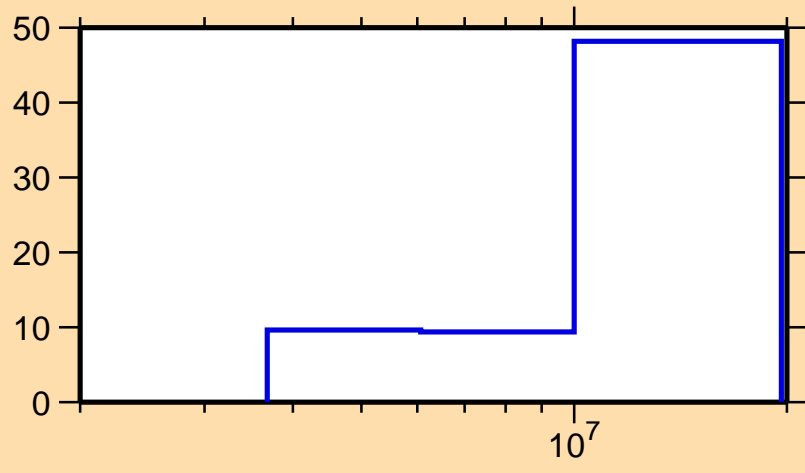
\Delta\sigma/\sigma vs. E for ^{63}\text{Co}(n,n\text{cont.})
