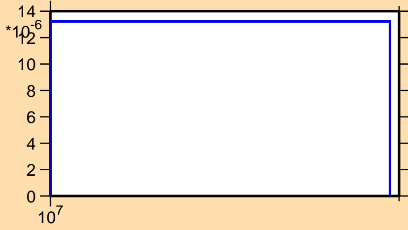
\sigma vs. E for ^{63}\text{Co}(n,t)
