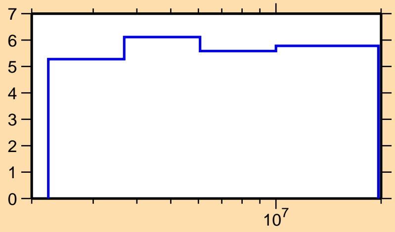
\Delta\sigma/\sigma vs. E for ^{63}\text{Co}(n,n\text{nonel.})
