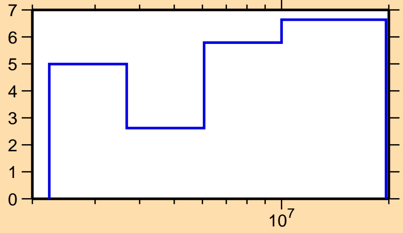
\Delta\sigma/\sigma vs. E for ^{63}\text{Co}(n,\text{tot.})
