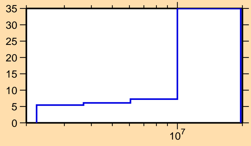
\Delta\sigma/\sigma vs. E for ^{63}\text{Co}(n,\text{inel.})
