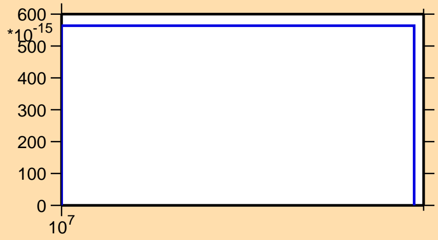
\sigma vs. E for ^{63}\text{Co}(n,2np)
