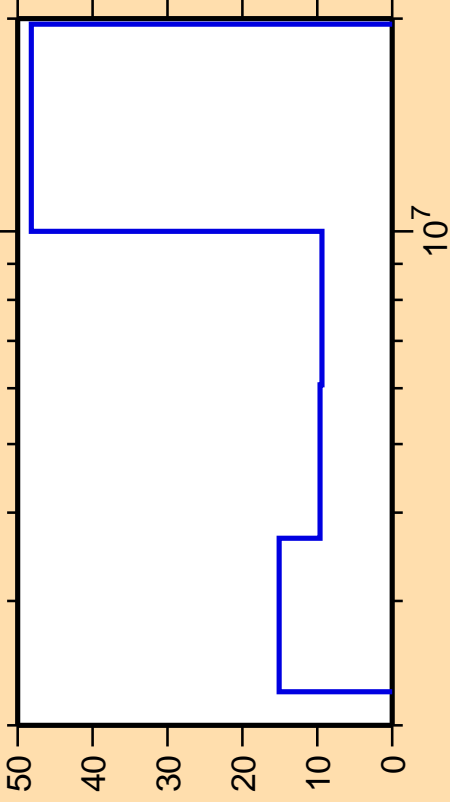
\Delta\sigma/\sigma vs. E for ^{63}\text{Co}(n,n\text{cont.})
