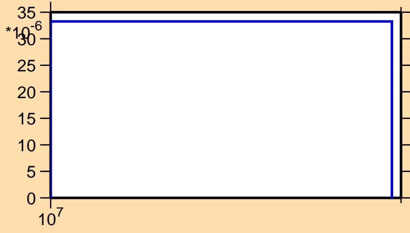
\sigma vs. E for ^{63}\text{Co}(n,n\alpha)
