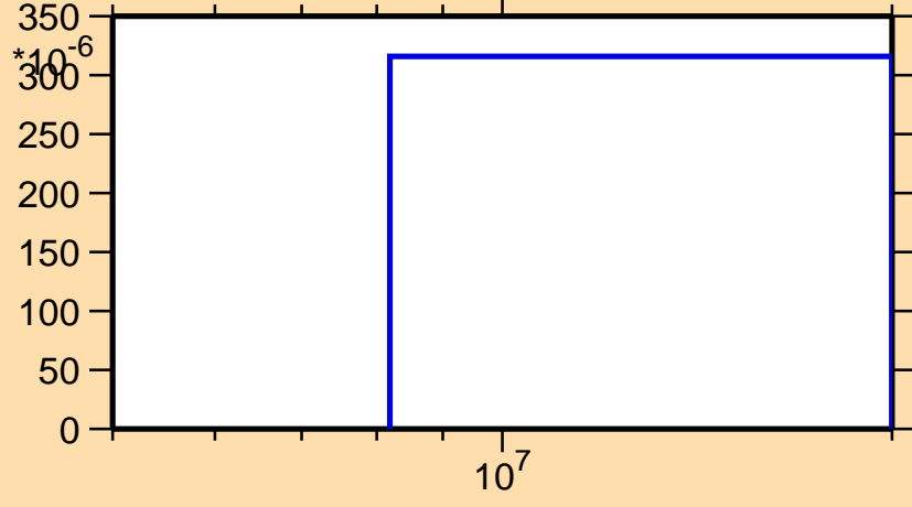
\sigma vs. E for ^{63}\text{Co}(n,np)
