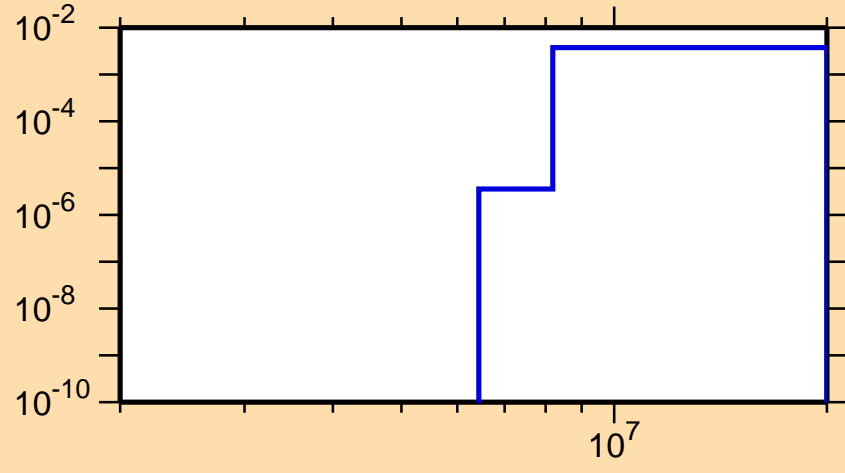
\sigma vs. E for ^{63}\text{Co}(n,p)
