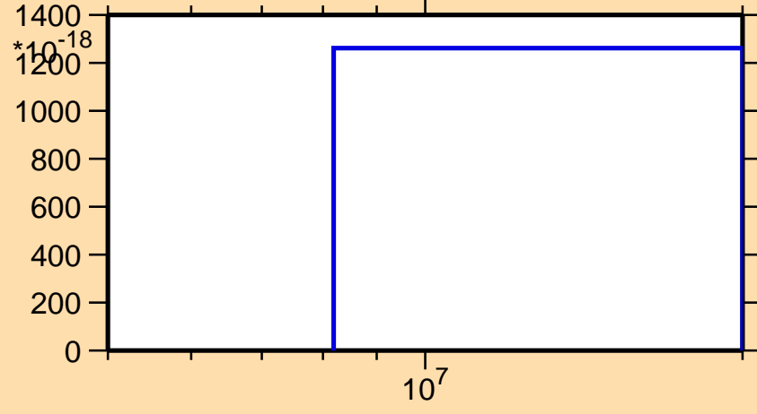
\sigma vs. E for ^{63}\text{Co}(n,2n\alpha)
