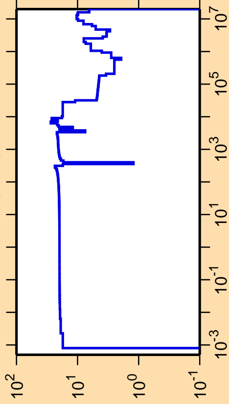
\Delta\sigma/\sigma vs. E for ^{65}\text{Co}(n,\text{el.})
