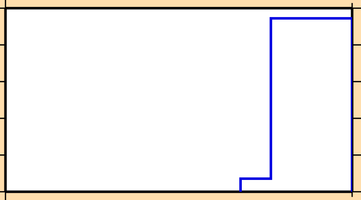
\sigma vs. E for ^{65}\text{Co}(n,nt)
