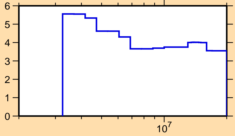
\Delta\sigma/\sigma vs. E for ^{65}\text{Co}(n,n\text{nonel.})
