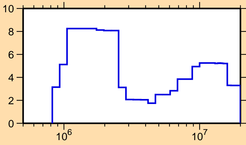
\Delta\sigma/\sigma vs. E for ^{65}\text{Co}(n,\text{tot.})
