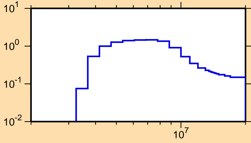
\sigma vs. E for ^{65}\text{Co}(n,n\text{cont.})
