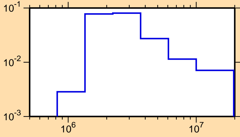
\sigma vs. E for ^{65}\text{Co}(n,n_3)
