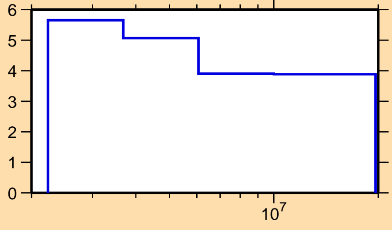
\Delta\sigma/\sigma vs. E for ^{65}\text{Co}(n,n\text{nonel.})
