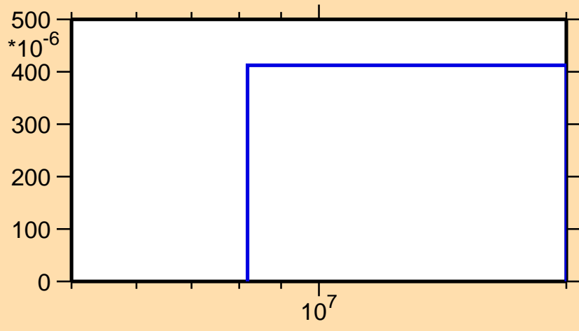
\sigma vs. E for ^{65}\text{Co}(n,d)
