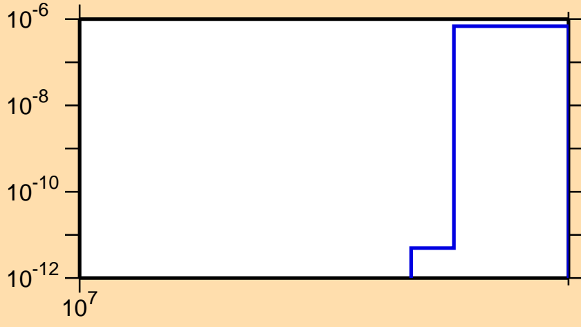
\sigma vs. E for ^{68}\text{Co}(n,nt)
