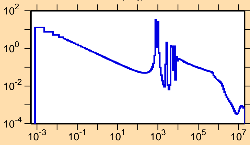
\sigma vs. E for ^{68}\text{Co}(n,\gamma)
