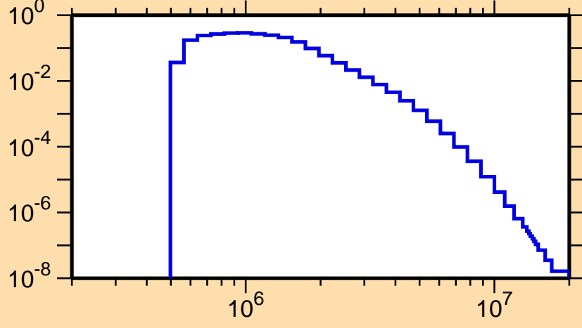
\sigma vs. E for ^{68}\text{Co}(n,n_3)
