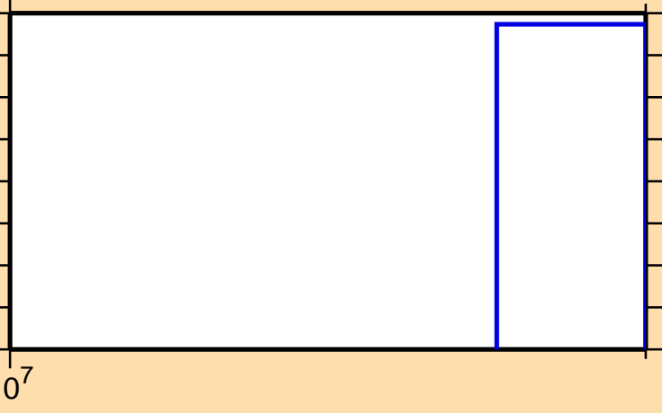
\sigma vs. E for ^{68}\text{Co}(n,2np)
