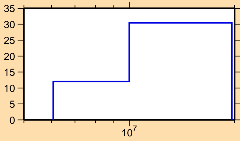
\Delta\sigma/\sigma vs. E for ^{68}\text{Co}(n,el.)
