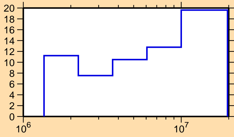
\Delta\sigma/\sigma vs. E for ^{68}\text{Co}(n,n\text{nonel.})
