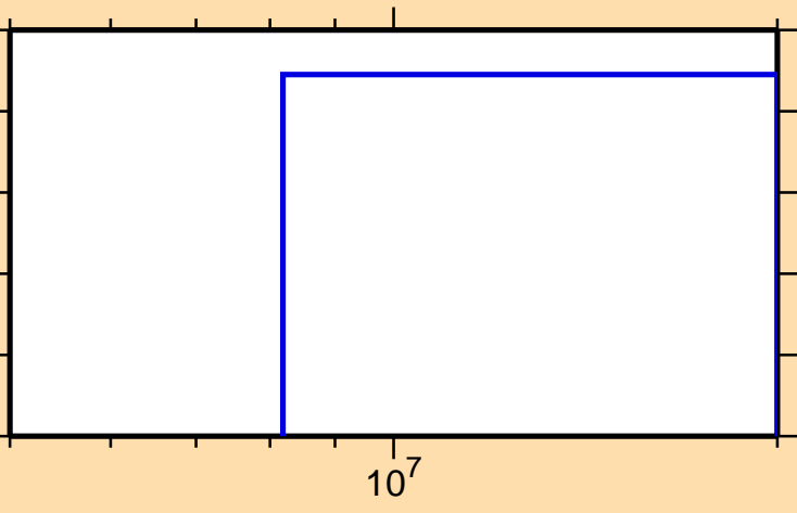
\sigma vs. E for ^{68}\text{Co}(n,t)
