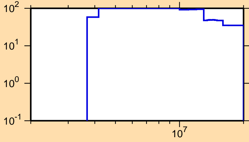
\Delta\sigma/\sigma vs. E for ^{48}\text{Cr}(n,n\text{cont.})
