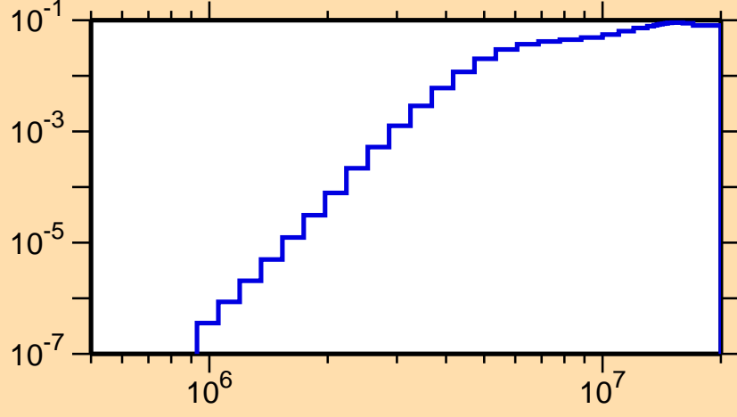
\sigma vs. E for ^{48}\text{Cr}(n,\alpha)
