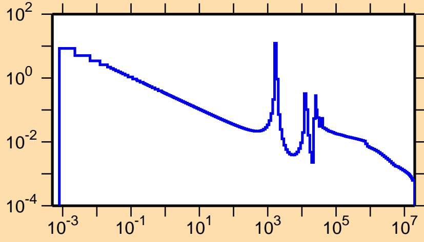
\sigma vs. E for ^{48}\text{Cr}(n,\gamma)
