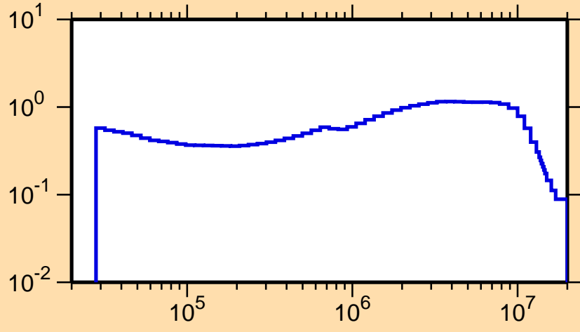
\sigma vs. E for ^{48}\text{Cr}(n,p)
