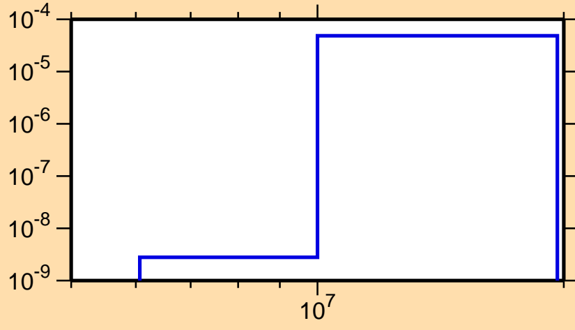
\sigma vs. E for ^{48}\text{Cr}(n,\text{He3})
