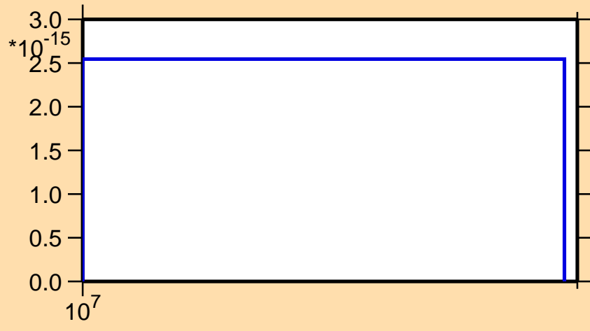
\sigma vs. E for ^{48}\text{Cr}(\text{mt117})
