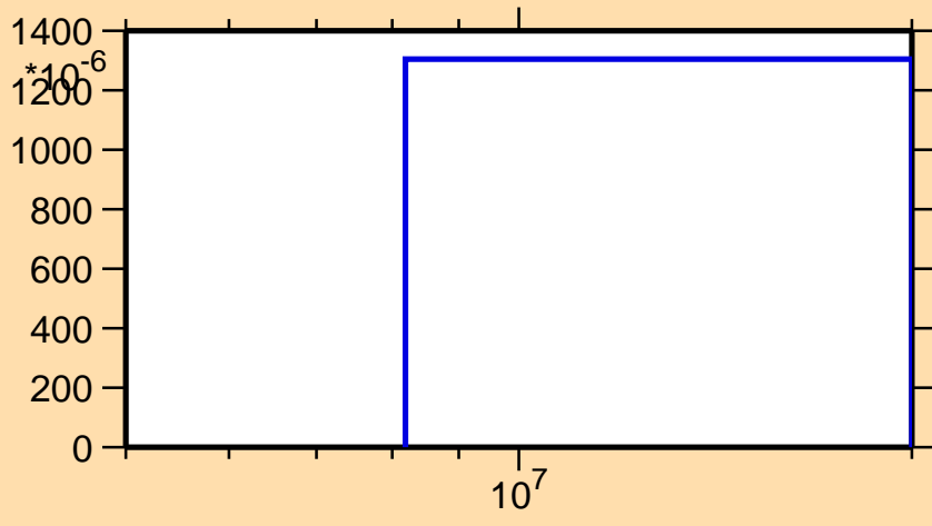
\sigma vs. E for ^{48}\text{Cr}(n,p\alpha)
