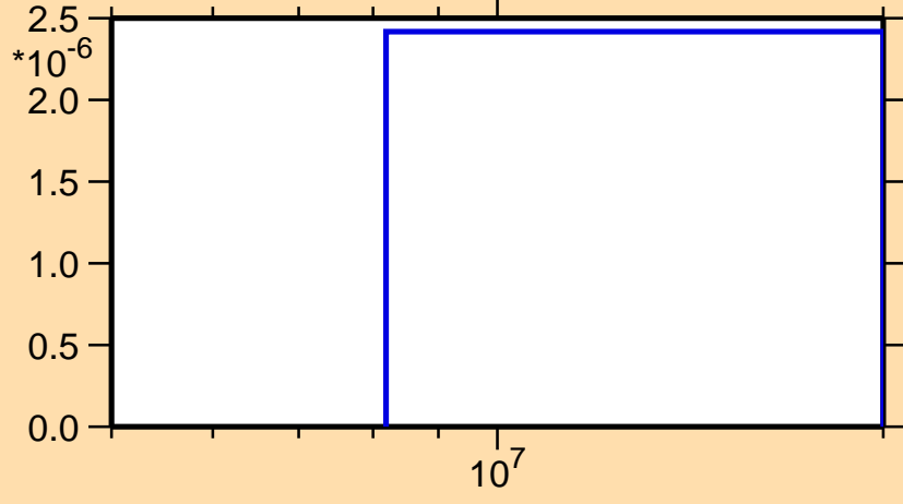
\sigma vs. E for ^{48}\text{Cr}(n,2n)
