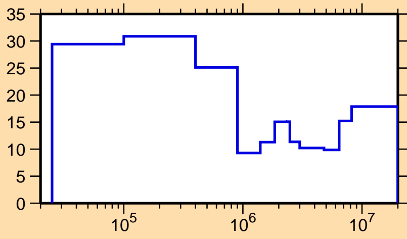
\Delta\sigma/\sigma vs. E for ^{48}\text{Cr}(n,el.)
