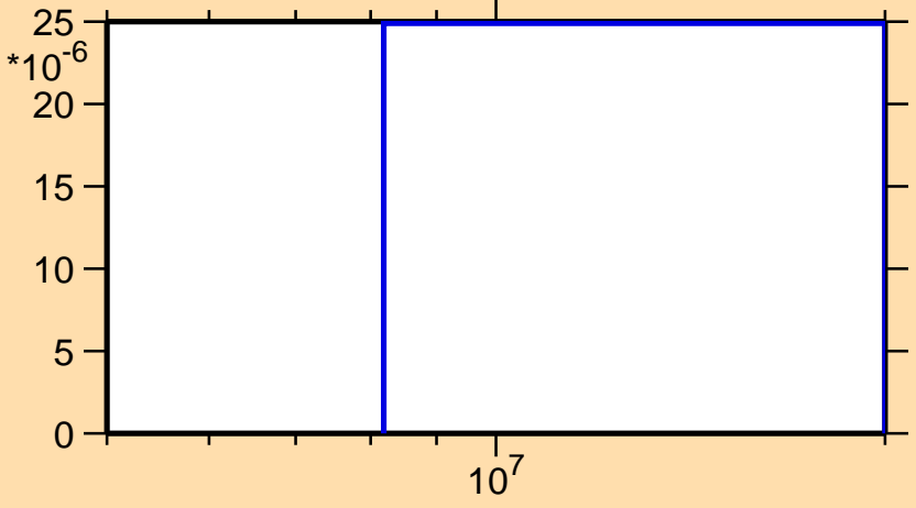
\sigma vs. E for ^{48}\text{Cr}(n,pd)
