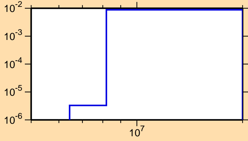
\sigma vs. E for ^{48}\text{Cr}(n,d)
