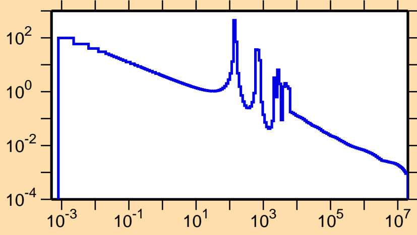
\sigma vs. E for ^{49}\text{Cr}(n,\gamma)
