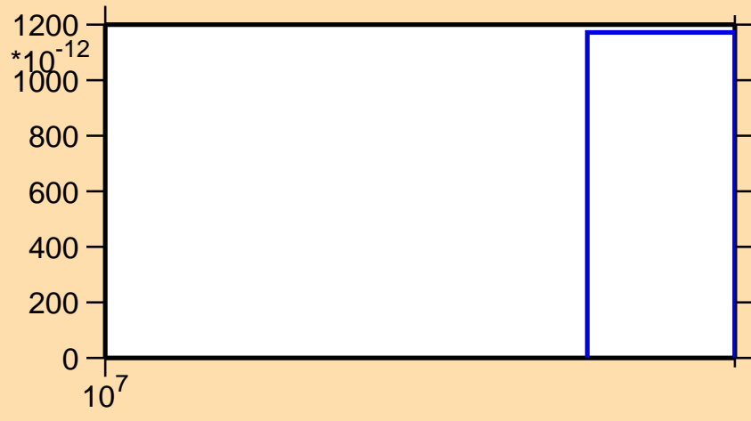
\sigma vs. E for ^{49}\text{Cr}(n,2np)
