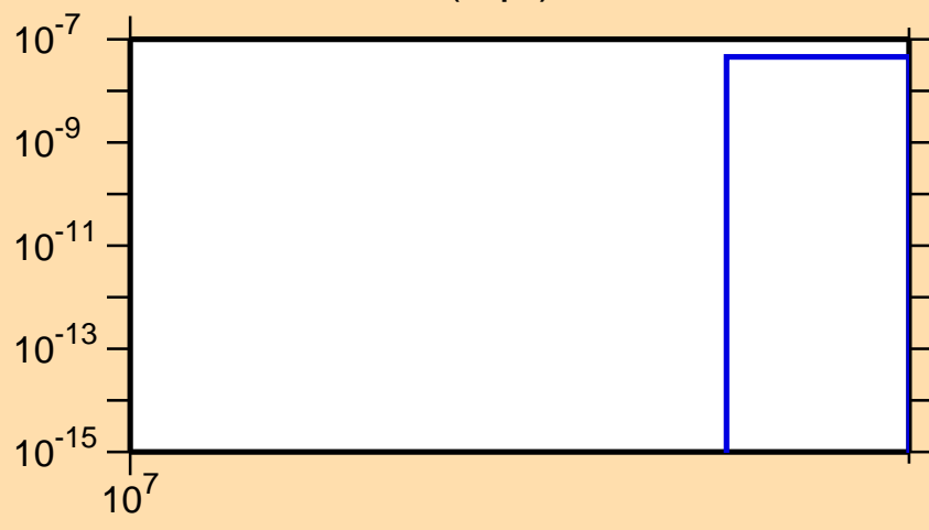
\sigma vs. E for ^{49}\text{Cr}(n,\text{pt})
