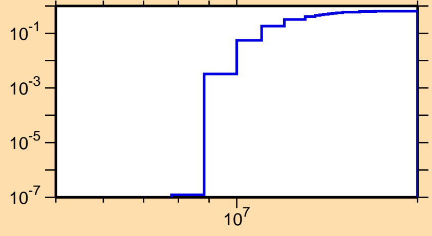
\sigma vs. E for ^{49}\text{Cr}(n,np)
