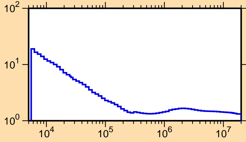
\sigma vs. E for ^{49}\text{Cr}(n,\text{nonel.})
