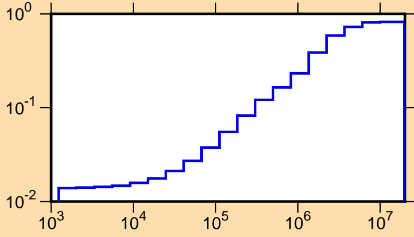
\mu vs. E for ^{49}\text{Cr}(\text{mt251})
