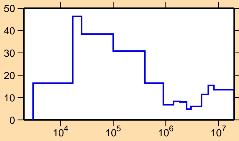
\Delta\sigma/\sigma vs. E for ^{49}\text{Cr}(n,el.)
