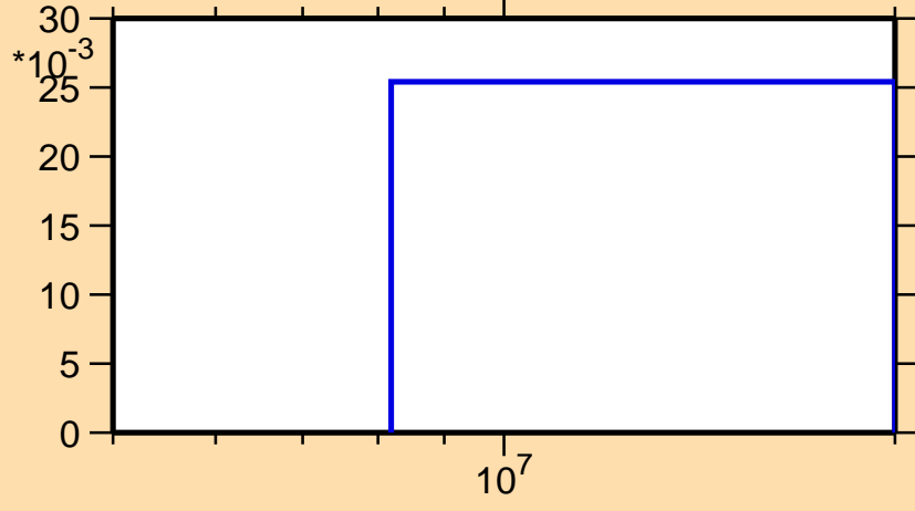
\sigma vs. E for ^{49}\text{Cr}(n,2n)
