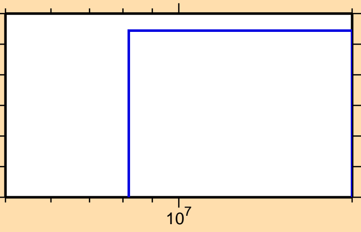
\sigma vs. E for ^{49}\text{Cr}(n,\text{nd})
