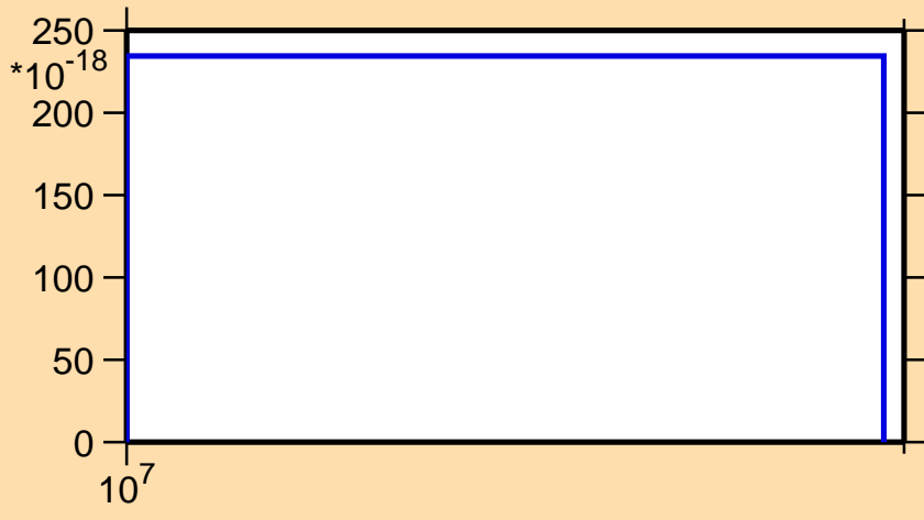
\sigma vs. E for ^{50}\text{Cr}(n,nd)
