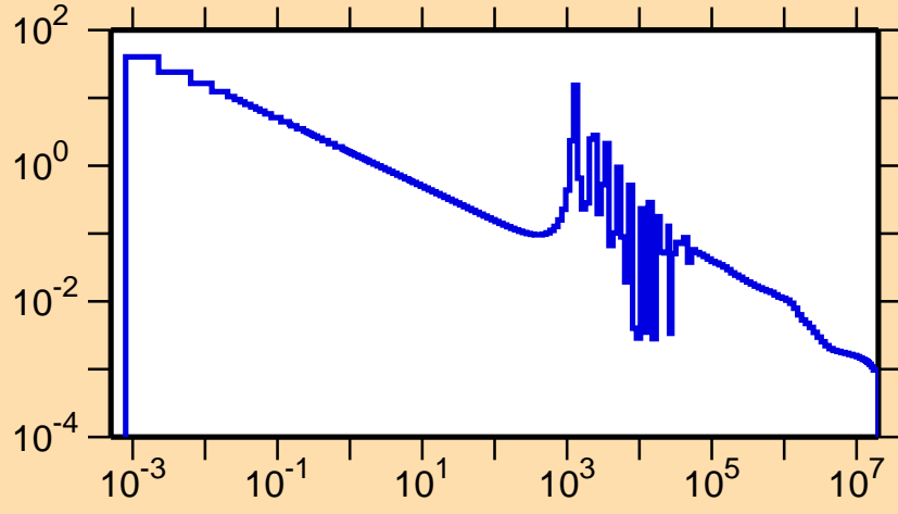
\sigma vs. E for ^{51}\text{Cr}(n,\gamma)
