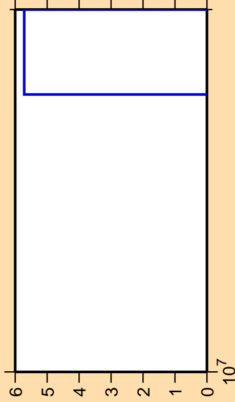
\Delta\sigma/\sigma vs. E for ^{51}\text{Cr}(n,\text{pt})
