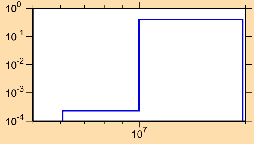
\sigma vs. E for ^{51}\text{Cr}(n,2n)
