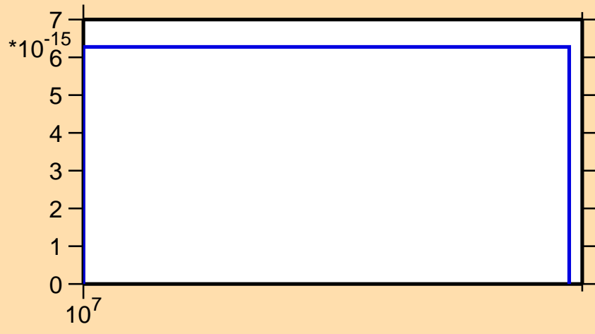
\sigma vs. E for ^{51}\text{Cr}(n,\text{pt})
