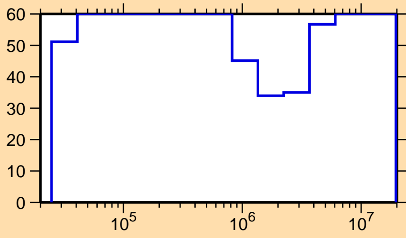
\Delta\sigma/\sigma vs. E for ^{51}\text{Cr}(n,p)
