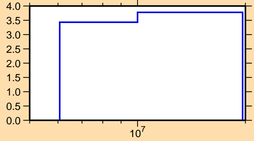
\Delta\sigma/\sigma vs. E for ^{51}\text{Cr}(n,\text{nonel.})
